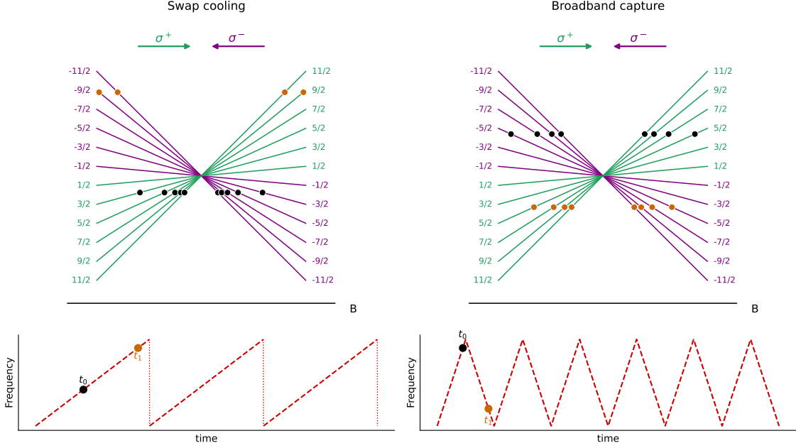
Figure 1.14: Sequential stages of the 689 nm red MOT. From left to right : swap cooling and broadband capture (adapted from [30]). The size of the cloud is decreasing with the cooling since the atoms are kicked in the opposite direction of the resonant laser of right polarization.
