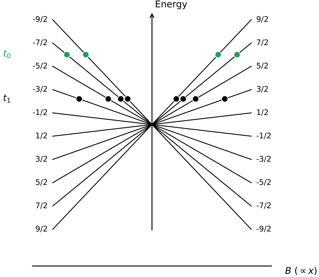
Figure 1.13: Spatial dependence of the resonance condition on each m_F sub-level, as a function of position x ( B \propto x ) – adapted from the principle illustrated in Fig. 2.8(d) of [30]. Right: the stirring laser’s frequency, swept in a sawtooth pattern over time in our implementation. At each instant t_0 , the instantaneous frequency (right) is simultaneously resonant with several (m_F, x) pairs (left, black dots); sweeping this frequency over time thus randomizes the m_F population across the whole trap.
