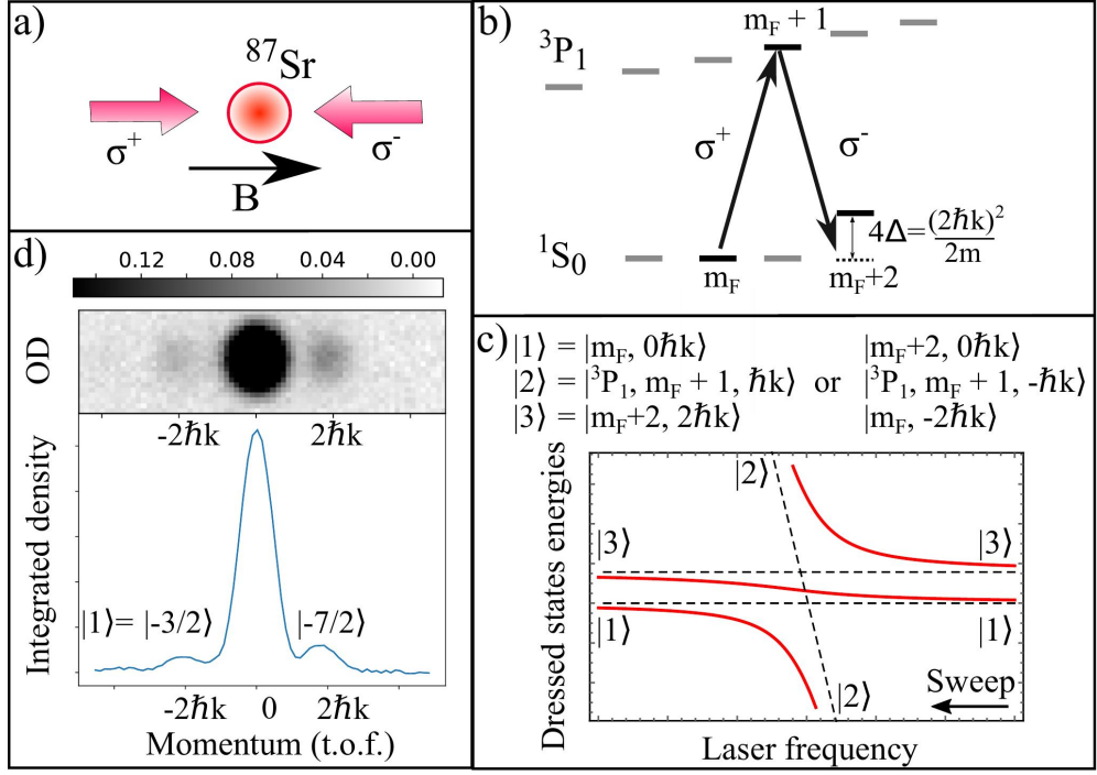
Figure 1.27: Principle of spin-selective detection via coherent momentum transfer. (a) Counter-propagating beam geometry of the lasers used for the TLS and two-photon Raman scheme. (b) Energy levels scheme of the Raman process, with recoil energy shifting the m_F + 2 level. (c) Avoided crossing due to the coupling of the states, necessitating adiabatic transfer. (d) Resulting TOF absorption image showing spatially separated spin components and the corresponding momentum distribution.
