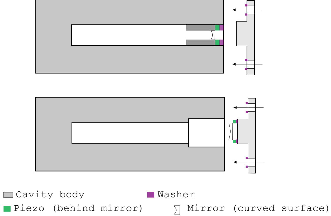
Figure 1.22: Top : Initial fixed cavity assembly using glued mirrors, lacking mechanical alignment degrees of freedom. Bottom : Upgraded and final cavity mount featuring three adjustment screws and compliant washers for precise angular and longitudinal alignment
