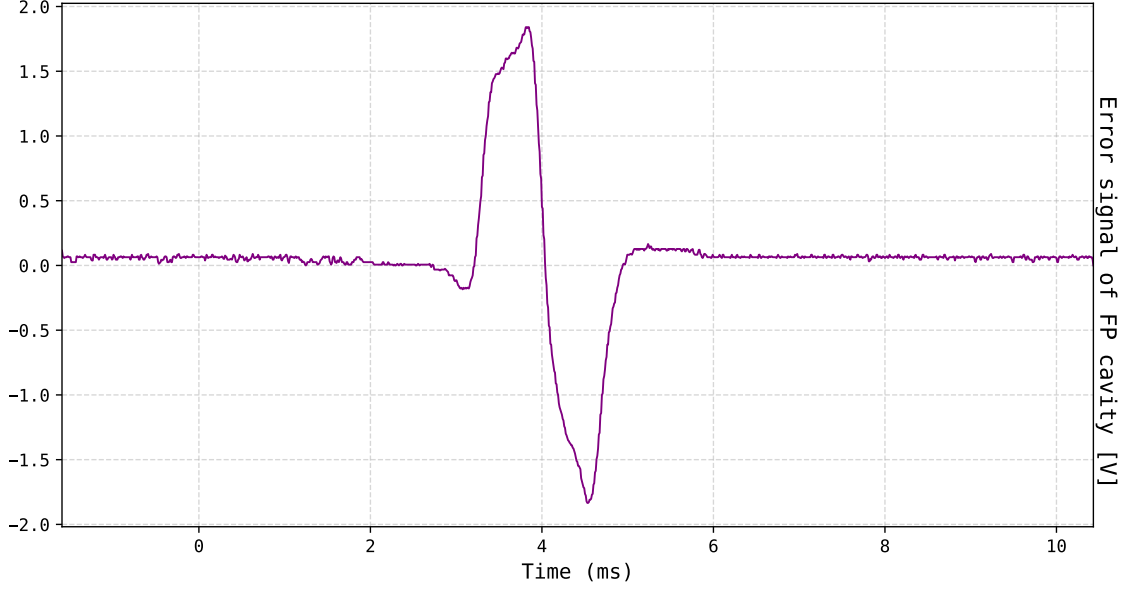
Figure 1.24: Pound-Drever-Hall (PDH) error signal obtained by scanning the cavity length across resonance, enabling the lock cavity for the filtering of MOGLabs laser.
