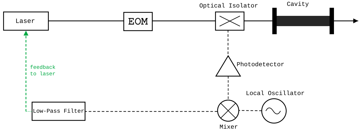
Figure 1.23: Schematic of the Pound-Drever-Hall locking system, extracted and adapted from [32]. The laser is firstly passing through an EOM that is modulating the electric field at frequency f_M , creating two sidebands at frequency f_{\text{laser}} \pm f_M . The carrier at f_{\text{laser}} and the sidebands are passing through the filtering Fabry-Pérot cavity which is reflecting the light going back to the entrance of the cavity. A beamsplitter serving as an optical isolator is reflecting the light to a photodiode. Then this signal is mixed with a local oscillator to extract an error signal to which a low-pass filter is combined to keep only the signal for the locking.
