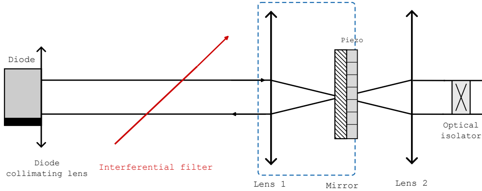
Figure 1.19: MOGlabs External Cavity Diode Laser (ECDL) architecture used for spin manipulation. A diode lasing at 689 nm is first collimated by a lens, then its frequency is roughly selected by an interference filter marked in red. The beam is focused by a second lens onto a partially reflective mirror (hatched rectangle): together they form a cat’s-eye retroreflector that closes the external cavity, feeding most of the light back for resonant frequency filtering while transmitting a small fraction onward. This output is collimated by a last lens and leaves the laser head through an optical isolator.
