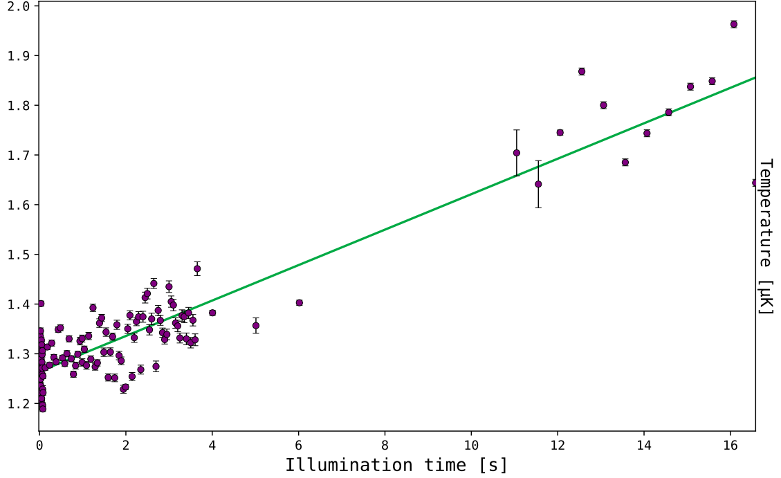
Figure 3.21: Temperature of the gas during the experiment described in Fig. ?, where the atom number decays with a two-body-loss-like behavior despite the signal being of atomic, not molecular, origin. The temperature increases linearly rather than following the saturating exponential expected for genuine photoassociative (two-body) loss, consistent with ordinary photon-scattering heating rather than molecule formation.
