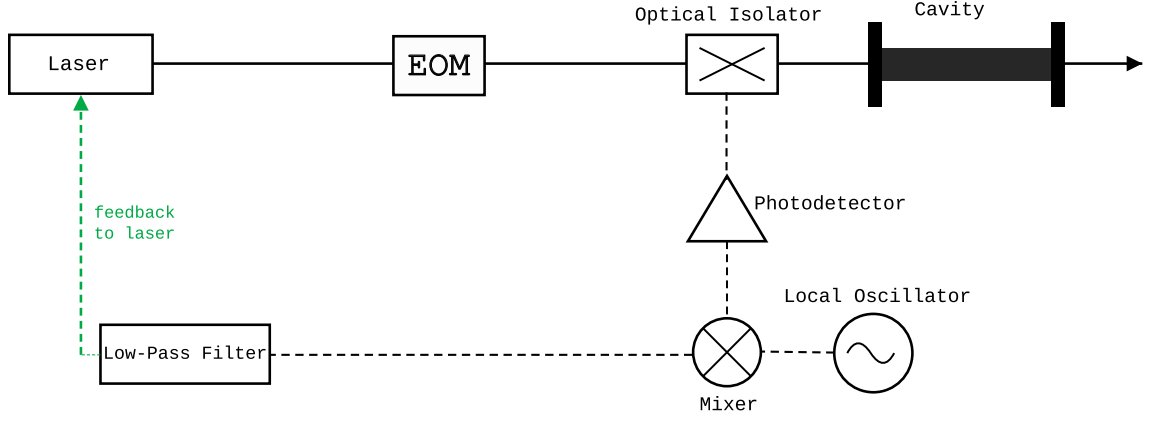
Figure 1.24: Schematic of the Pound-Drever-Hall locking system, extracted and adapted from [? ]. The laser is firstly passing through an EOM that is modulating the electric field at frequency f_M , creating two sidebands at frequency f_{laser} \pm f_M . The carrier at f_{laser} and the sidebands are passing through the filtering Fabry-Pérot cavity which is reflecting the light going back to the entrance of the cavity. A beamsplitter serving as an optical isolator is reflecting the light to a photodiode. Then this signal is mixed with a local oscillator to extract an error signal to which a low-pass filter is combined to keep only the signal for the locking.
