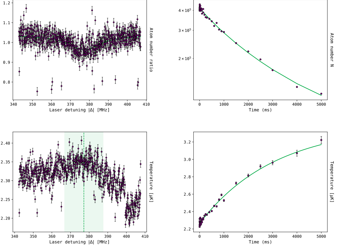
Figure 3.24: Characterization of the molecular line at 375.74 \pm 0.48 MHz in ^{87}\text{Sr} . Panel layout as in Fig. ??, with I = 19 W/cm 2 for the N(t)/T(t) fits. All detunings are measured from the ^{87}\text{Sr} atomic resonance.
