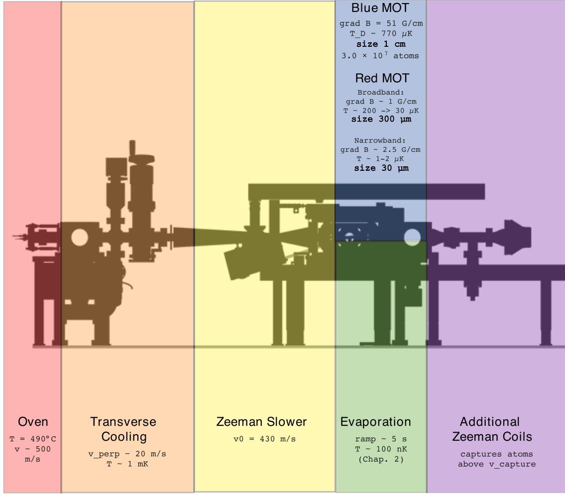
Figure 1.2: Extracted and modified from [?] Experimental full setup for the cooling and trapping of the atoms with figures on the velocity, temperature and typical magnetic gradient on each stage.
