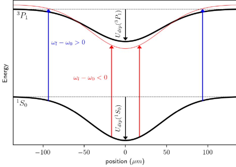
Figure 1.15: Simulation extracted from [? ]. Principle of localized 689 nm MOT loading inside the crossed optical dipole trap due to the differential AC Stark shift between ^1S_0 and ^3P_1 .
