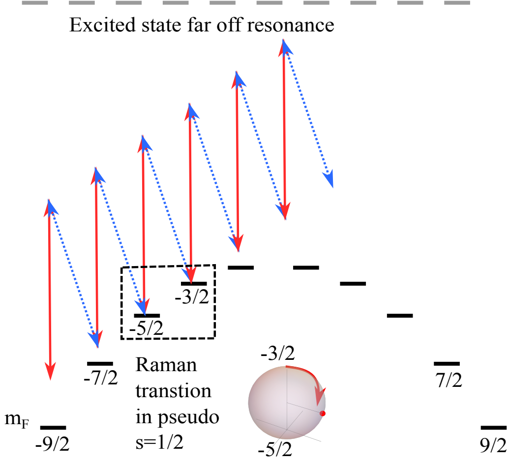
Figure 1.20: Spin manipulation scheme of [? ]. The isolation of spin states is allowed by the tensorial shift of the ground states that makes neighbours m_F states isolated from the other resonances.
