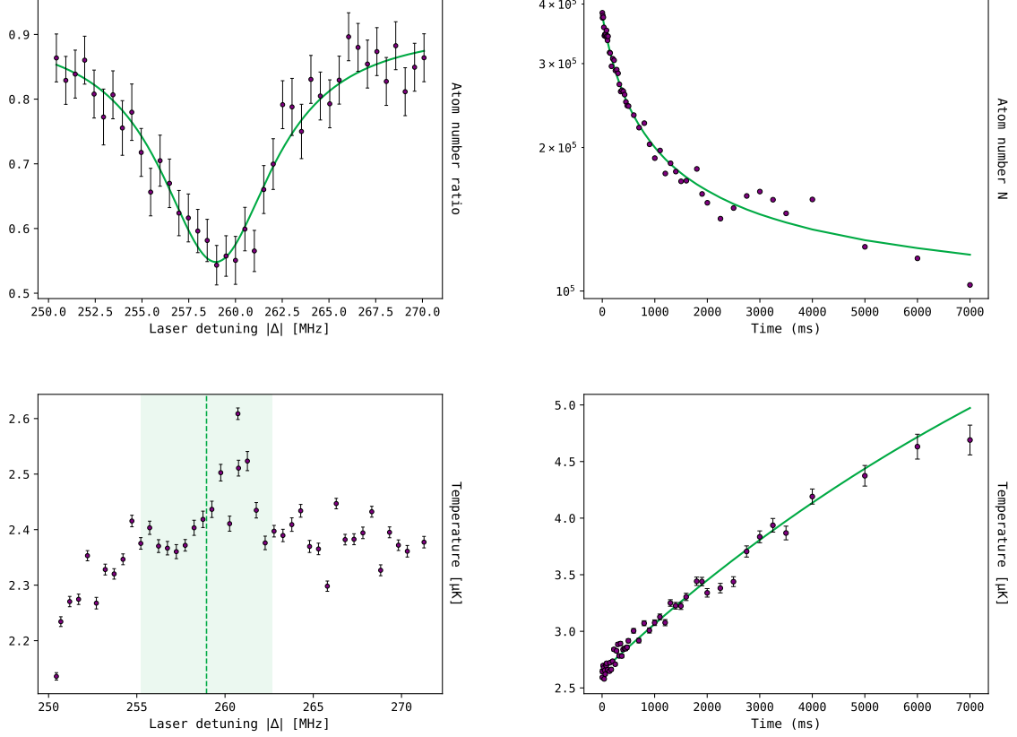
Figure 3.22: Characterization of the molecular line at 259.01 \pm 0.12 \text{ MHz} in ^{87}\text{Sr} . Top left: resonance spectrum ( I = 19 \text{ W/cm}^2 , t = 1000 \text{ ms} ), with Lorentzian fit (green). Top right: atom number decay N(t) , fitted via Eq. ?? with interpolated T(t) . Bottom left: temperature of the cloud versus detuning; the shaded region and dashed line mark the resonance width and center from the top-left fit. Bottom right: temperature versus illumination time, with a saturating-exponential fit ( \Gamma fixed to the N(t) value). All detunings are measured from the ^{87}\text{Sr} atomic resonance.
