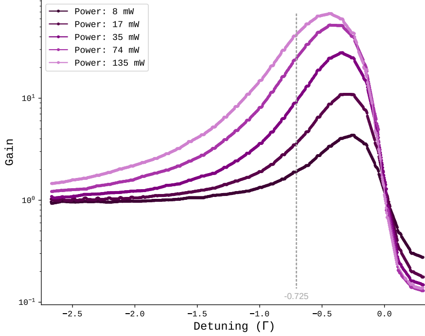
Figure 1.7: Transverse cooling performance as a function of laser detuning and power (adapted from [? ]). Curves of atom number gain for different optical powers on TC are showing optimum that are not centered on the same detuning.
