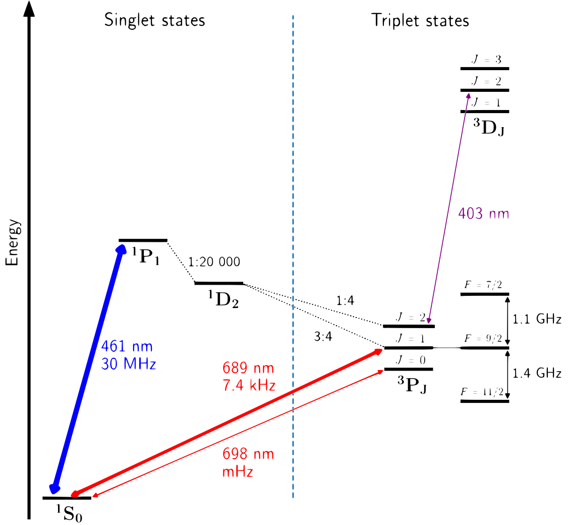
Figure 1.1: Extracted from [?] Energy spectrum of ^{87}\text{Sr} including fine and hyperfine interactions. In blue the 461 nm transition used for TC, Zeeman cooling, blue MOT stage and imaging. The purple arrow indicates the repump line at 403 nm from the metastable state ^3P_2 used for the atoms leaking from the intermediate ^1D_2 state. In red the transition to ^3P_1 at 689 nm used for all stages of the red MOT, optical pumping, spin manipulation, coherent manipulation (see Chap.??), photoassociation (see Chap.??, through the different hyperfine states F = 7/2, 9/2, 11/2 ). The 698 nm transition indicates the clock transition which we do not use in this experiment.
