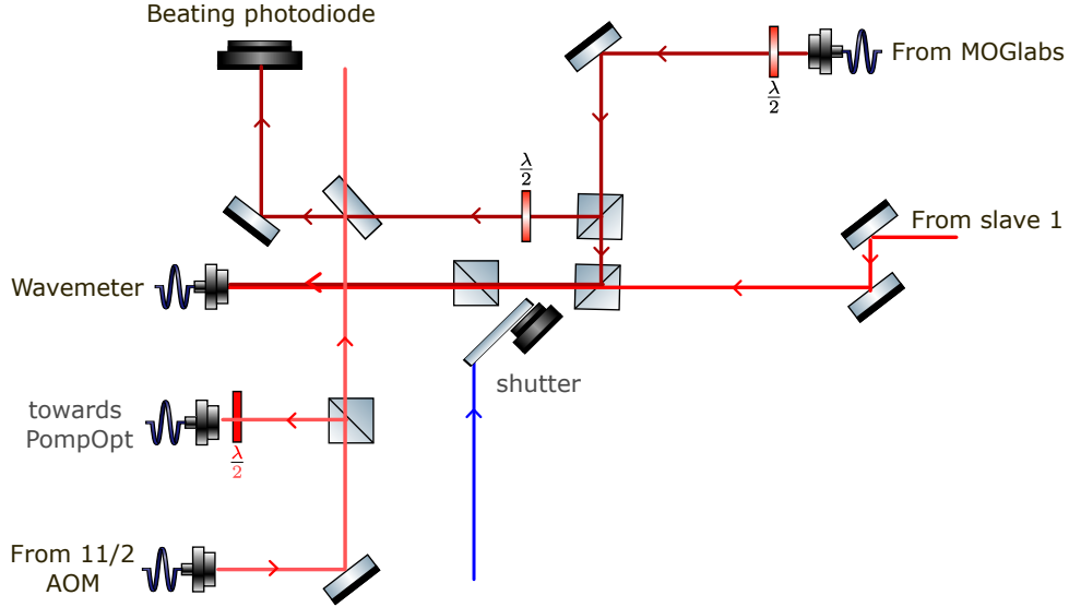
Figure 3.8: Beating scheme for PA process between the light from "AOM 11/2" that is settled on the resonance ^1S_0 \rightarrow ^3P_1, F = 11/2 , and MOGlabs. The light is coming from ?? to split in two arms: optical pumping and PA. This last one serves for MOGlabs locking in a beating procedure where the beam is recombined by the 50/50 waveplate superposing with slave 1 beam.
