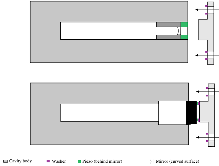
Figure 1.23: Top : Initial fixed cavity assembly using glued mirrors, lacking mechanical alignment degrees of freedom. Bottom : Upgraded and final cavity mount featuring three adjustment screws and compliant washers for precise angular and longitudinal alignment
