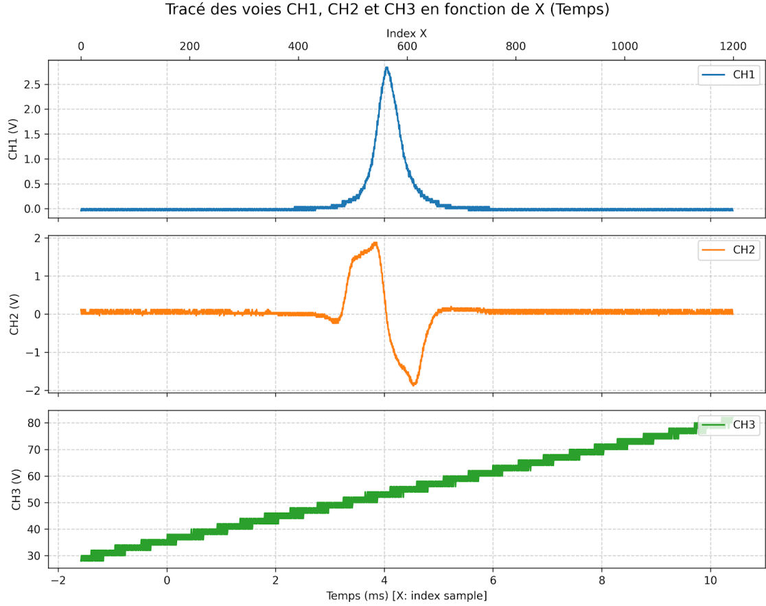
Figure 1.24: Typical Pound-Drever-Hall (PDH) error signal obtained by scanning the cavity length across resonance.
