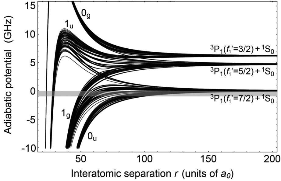
Figure 3.7: Density of molecular potentials for ^{173}\text{Yb} with three hyperfine states enhancing numerous triplet of quantum numbers (T, F, R) . The spectral lines are identified by S_{u/g} with S the total orbital momentum of the molecule and u/g the parity of the electronic wavefunction (see 3.3).
