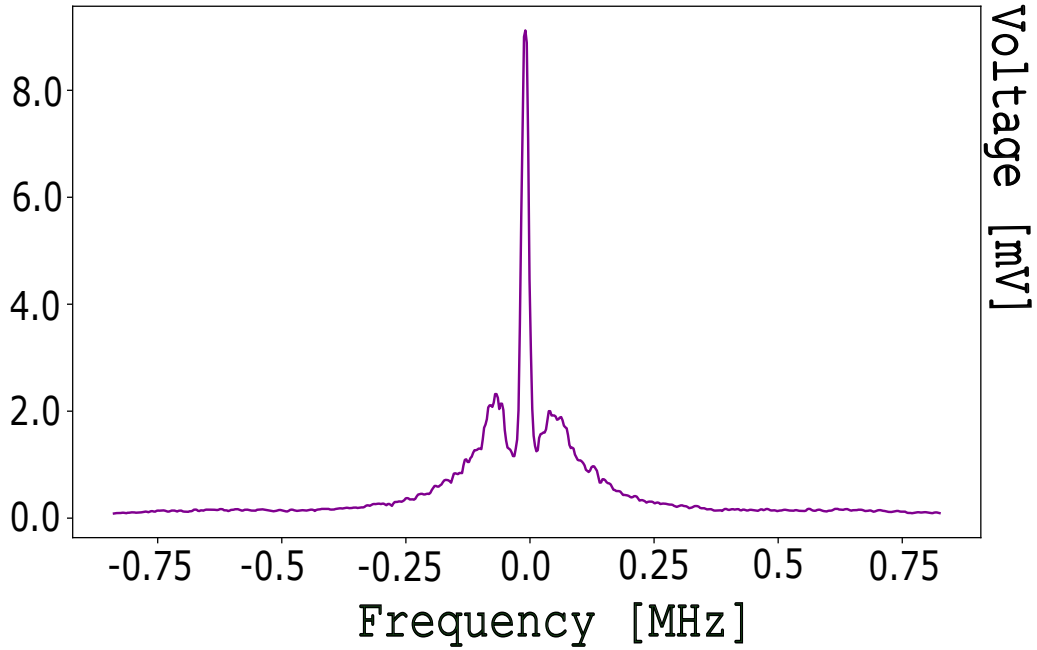
Figure 3.12: Beating spectrum between the MOGlabs laser and the "AOM 11/2" measured at the spectrum analyzer at \text{RBW} = 10\text{ kHz} and \text{VBW} = 300\text{ Hz} . The side components at around \pm 50\text{ kHz} induce a broadening of the natural linewidth of atoms/molecules addressed by the PA beam coming from the MOGlabs head beat locked.
