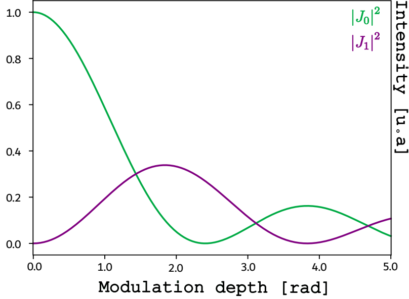
Figure 3.13: Modulus square of the 0^{th} and 1^{st} Bessel functions J_n governing the power distribution between the carrier and PDH sidebands.
