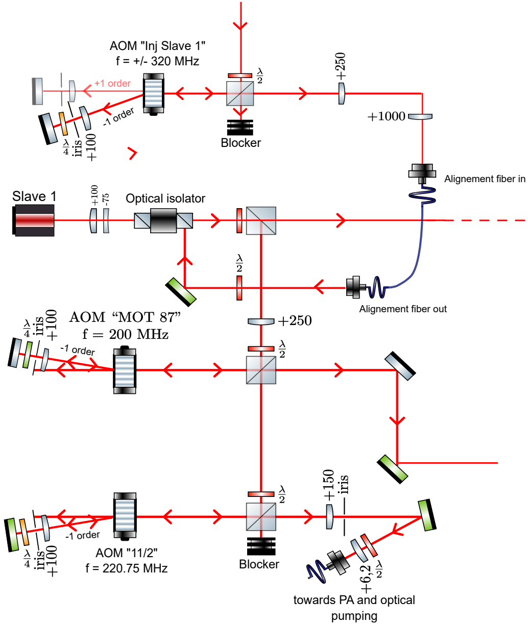
Figure 3.21: Zoom on the section of the red chain dedicated to the PA process. The frequency for both laser configurations is tuned by "AOM Inj Slave 1", adjusted by "AOM 11/2" before being sent to the atoms.
