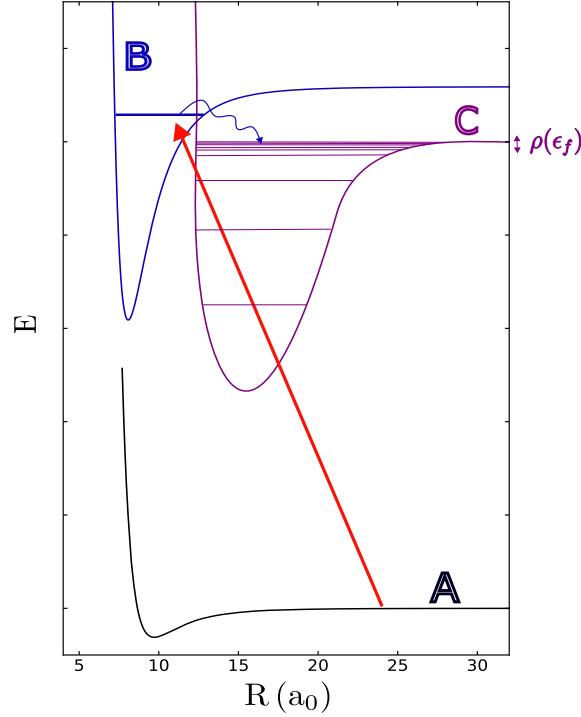
Figure 3.27: Scheme of predissociation which is a phenomenon that occurs when dissociation limit of an excited molecular potential C is under the closed channel of the excited molecule of potential B. Then the \nu_B state is coupled to a density of states of potential C that modifies the linewidth \Gamma_{mol} of the molecular state
