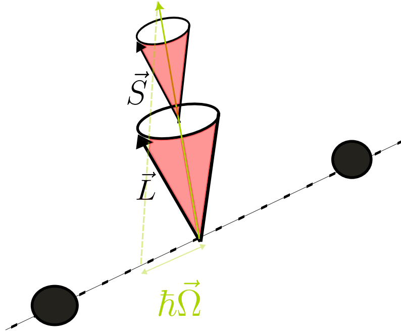
Figure 3.5: Hund case (c) is a case where spin-orbit coupling dominates the interaction, resulting in a angular momenta of projection \hbar\Omega in internuclear axis. In this case we took R = 0 as in many cases.
