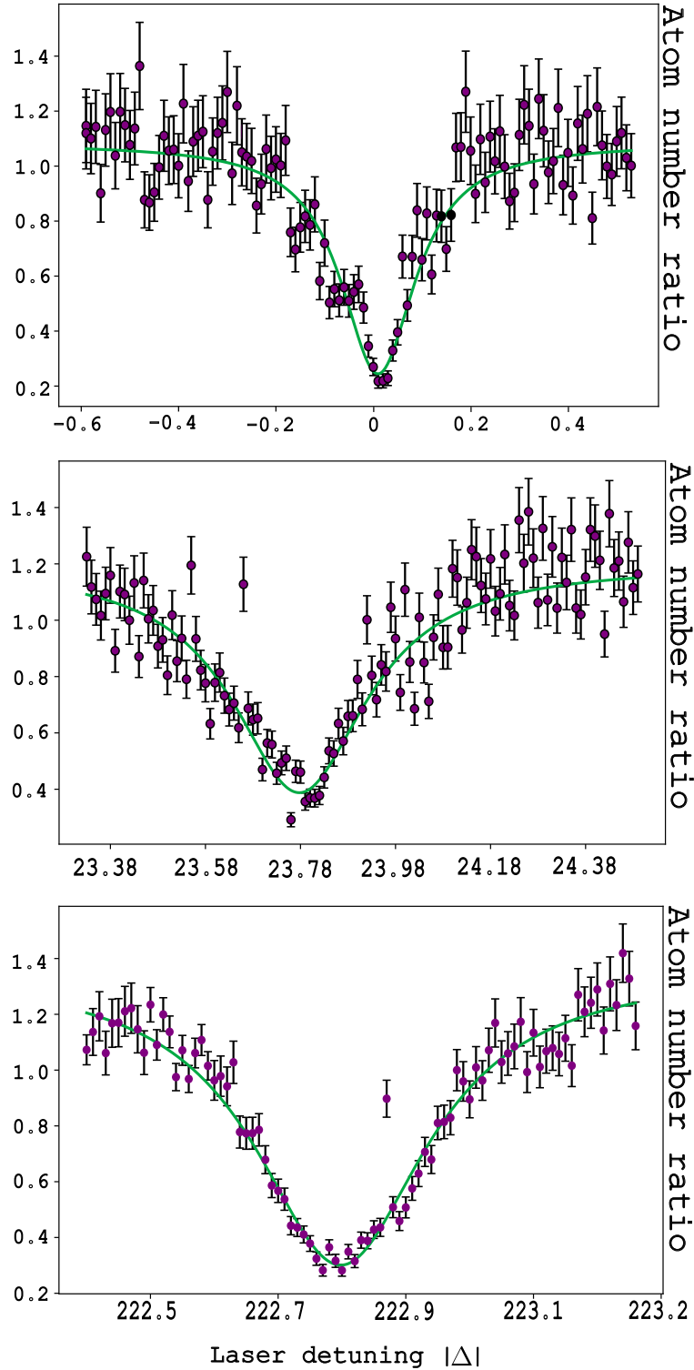
Figure 3.16: Normalized ^{88}\text{Sr} atom number across the intercombination line. (Top) Atomic resonance used as the PA frequency reference. Data points are extracted from 2D Gaussian fits of absorption images; error bars include fit covariance and unperturbed cloud RMS fluctuations. (Middle) \nu = -1 vibrational state ( I = 826 \text{ mW/cm}^2 , 1000 ms). (Bottom) \nu = -2 vibrational state ( I = 303 \text{ mW/cm}^2 , 50 ms). Solid lines are Lorentzian fits with errors accounting for covariance and systematic fluctuations.
