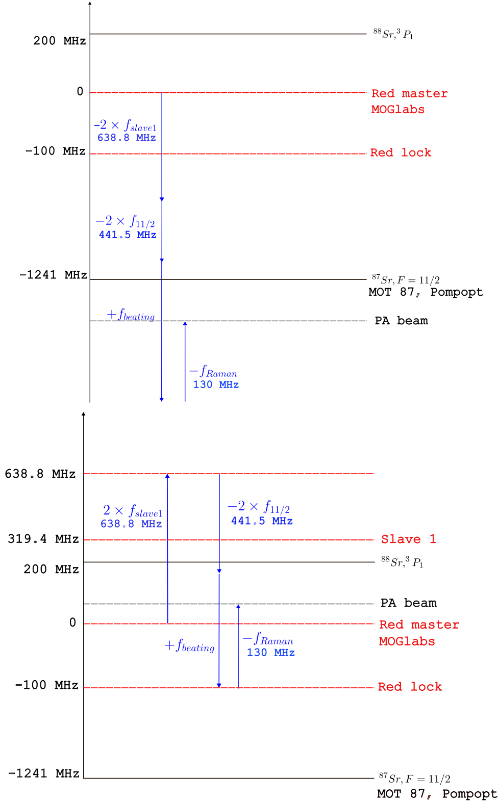
Figure 3.11: Frequency schemes for photoassociation (PA) depending on the targeted isotope: (top) scheme for ^{87}\text{Sr} and (bottom) scheme for ^{88}\text{Sr} . Switching the diffracted order of 'AOM Slave 1' allows for a seamless transition between isotopes, requiring only a minor realignment of the beam injection downstream of the AOM.
