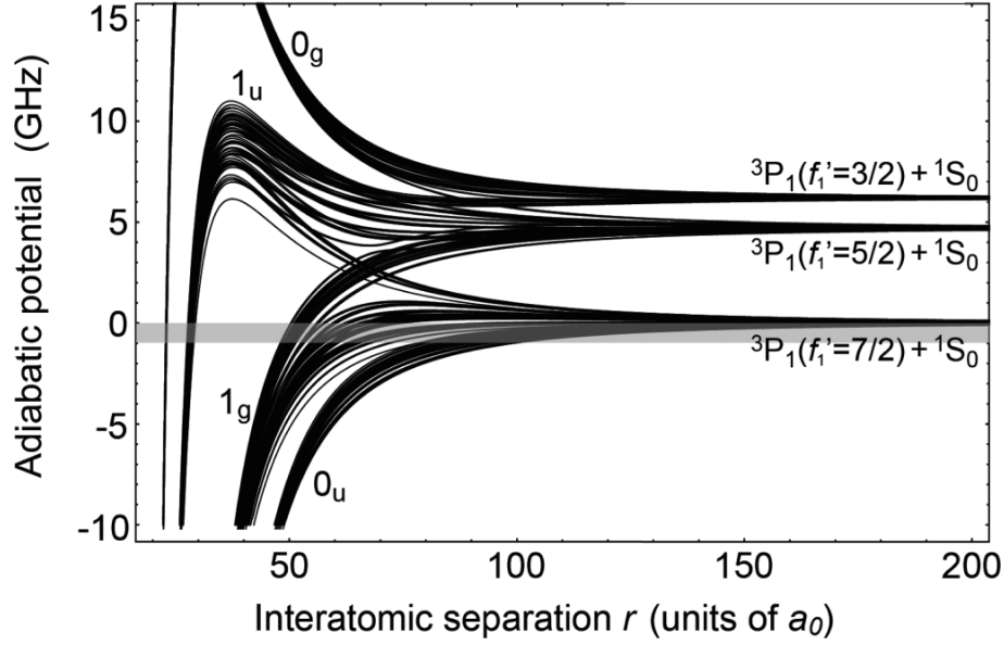
Figure 3.6: Density of molecular potentials for ^{173}\text{Yb} with three hyperfine states enhancing numerous triplet of quantum numbers ( T, F, R ). The spectral lines are identified by S_{u/g} with S the total orbital momentum of the molecule and u/g the parity of the electronic wavefunction (see 3.3).
