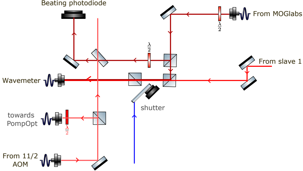
Figure 3.7: Beating scheme for PA process between the light from "AOM 11/2" that is settled on the resonance ^1S_0 \rightarrow ^3P_1, F = 11/2 , and MOGLabs. The light is coming from 3.18 to split in two arms: optical pumping and PA. This last one serves for MOGLabs locking in a beating procedure where the beam is recombined by the 50/50 waveplate superposing with slave 1 beam.
