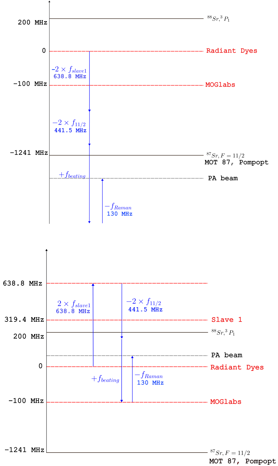
Figure 3.8: Frequency schemes for photoassociation (PA) depending on the targeted isotope: (top) scheme for ^{87}\text{Sr} and (bottom) scheme for ^{88}\text{Sr} . Switching the diffracted order of 'AOM Slave 1' allows for a seamless transition between isotopes, requiring only a minor realignment of the beam injection downstream of the AOM.
