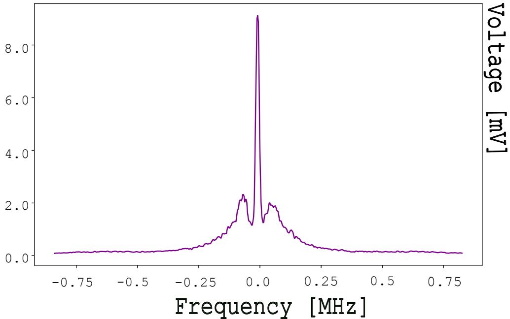
Figure 3.9: Beating spectrum between the MOGlabs laser and the "AOM 11/2" measured at the spectrum analyzer at \text{RBW} = 10 \text{ kHz} and \text{VBW} = 300 \text{ Hz} , with a three-Lorentzian fit (central peak + two sidebands at \pm 70 \text{ kHz} ). The sidebands, of larger FWHM than the central peak, carry the majority ( \simeq 69\% ) of the total optical power.
