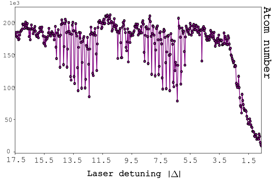
Figure 3.16: Twelve m_F states of the ^3P_1, F = 11/2 hyperfine excited state, measured in an SU(10) gas at \delta = -6 MHz and \delta = -12 MHz from the atomic resonance. This heating-broadened pattern of single-atom lines is displaced in frequency by a sideband in the diode laser spectrum.
