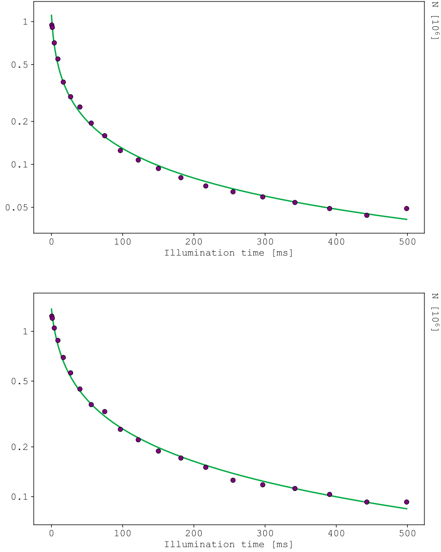
Figure 3.17: Top : atom number decay of ^{88}\text{Sr} of the resonance at f = -23.932(33) MHz. Bottom: atom decay of resonance at f = -222.79(1) MHz. Both plots use a logarithmic vertical scale. Solid lines: fit with two-body losses computed locally over the Gaussian density profile, without rethermalization, as expected for the nearly ideal ^{88}\text{Sr} gas [117]. The values of K_2 and l_{\text{opt}} given in the text were obtained with the global fit of the analysis software (Gaussian profile maintained); the local fit shown here gives a value larger by a factor \sim 2 , i.e. the same order of magnitude. Error bars are not shown, as the original raw data could not be recovered.
