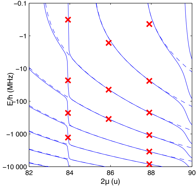
Figure 3.6: This graph - extracted from [14]- confronts the experimental internal states in red crosses to their theoretical predictions for different reduced mass of strontium isotopes. The theoretical model guarantees approximated scales for molecular lines of ^{87}\text{Sr} but not precisely because this model neglects the hyperfine interaction of the species.
