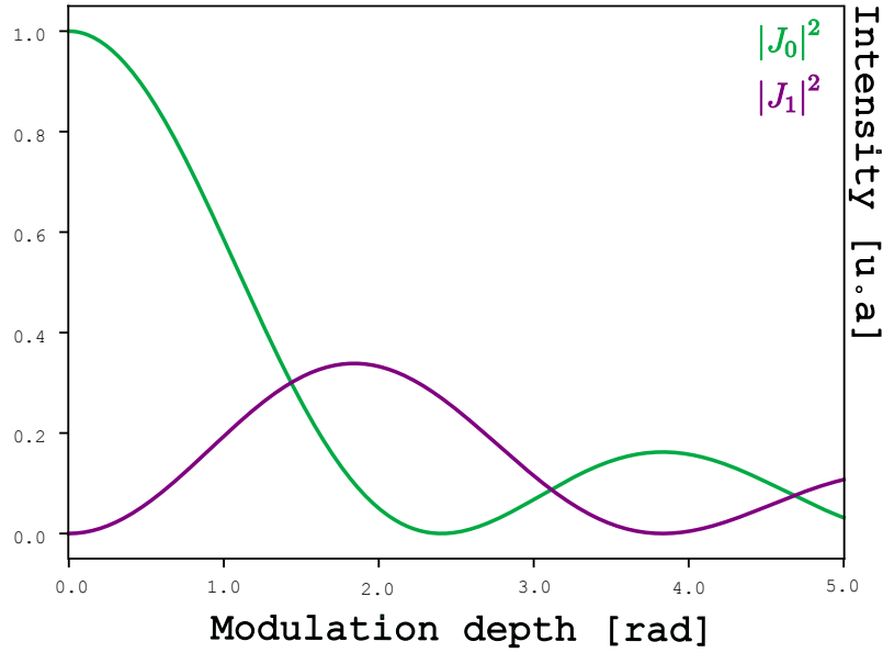
Figure 3.10: Modulus square of the 0^{th} and 1^{st} Bessel functions J_n governing the power distribution between the carrier and PDH sidebands.
