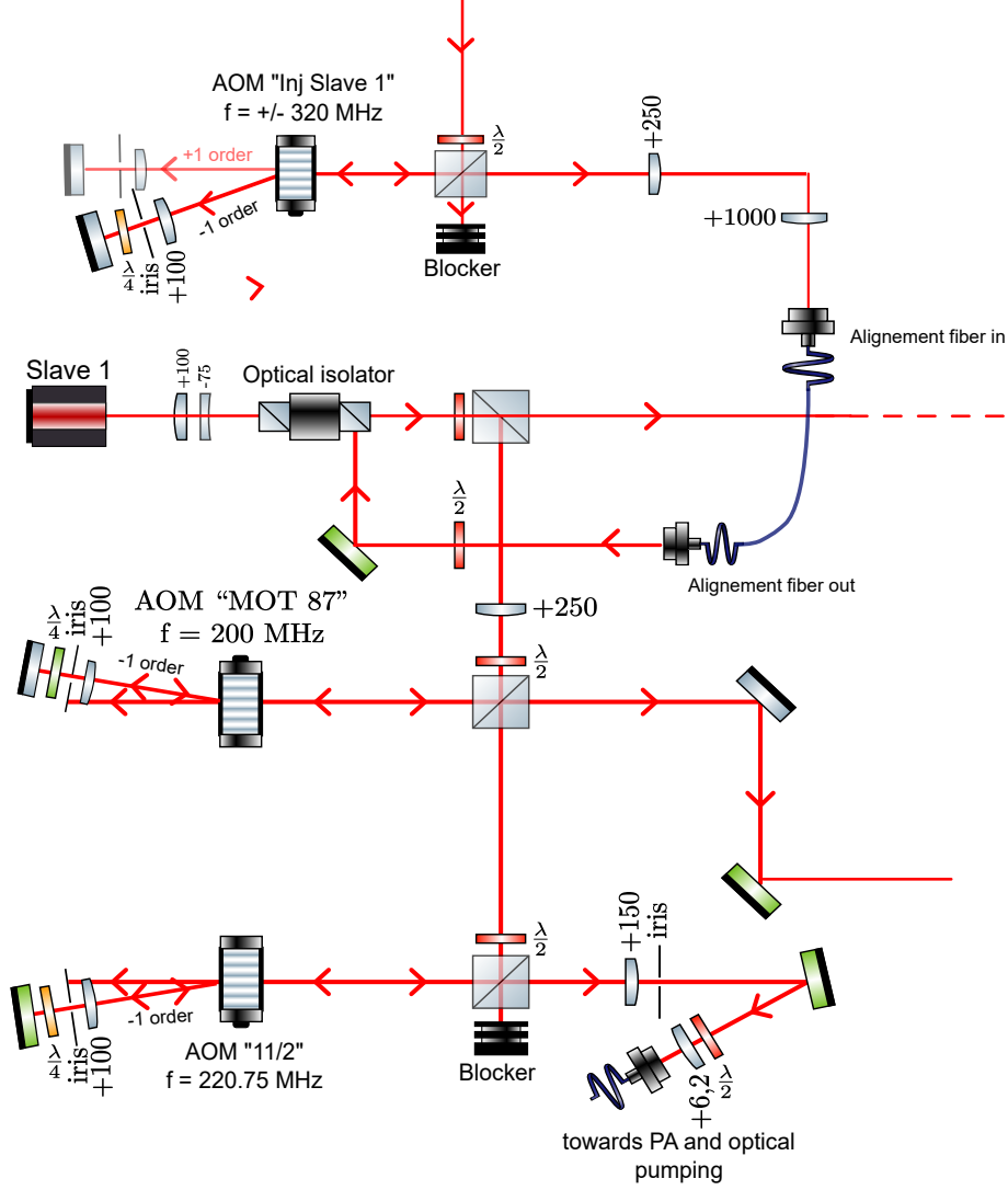
Figure 3.18: Zoom on the section of the red chain dedicated to the PA process. The frequency for both laser configurations is tuned by 'AOM Inj Slave 1', adjusted by 'AOM 11/2' before being sent to the atoms.
