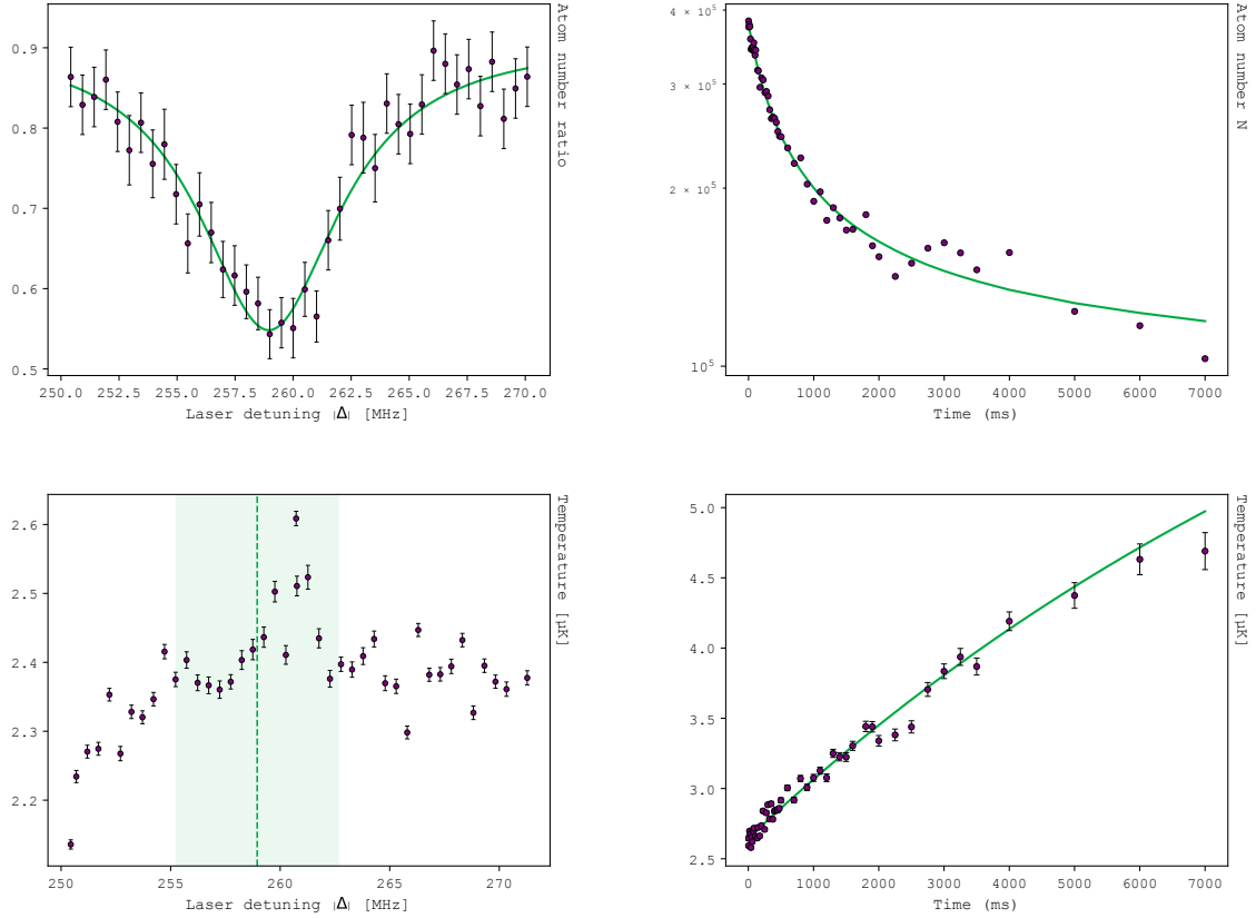
Figure 3.21: Characterization of the molecular line at 259.01 \pm 0.12 MHz in ^{87}\text{Sr} . Top left: resonance spectrum ( I = 19 \pm 1.1 W/cm 2 , t = 1000 ms, \langle n \rangle = (7.0 \pm 1.0) \times 10^{12} cm -3 ), with Lorentzian fit (green). Top right: atom number decay N(t) (same intensity and density), fitted via Eq. 3.82 with interpolated T(t) . Bottom left: temperature of the cloud versus detuning; the shaded region and dashed line mark the resonance width and center from the top-left fit. Bottom right: temperature versus illumination time, with a saturating-exponential fit ( \Gamma fixed to the N(t) value). All detunings are measured from the ^{87}\text{Sr} atomic resonance.
