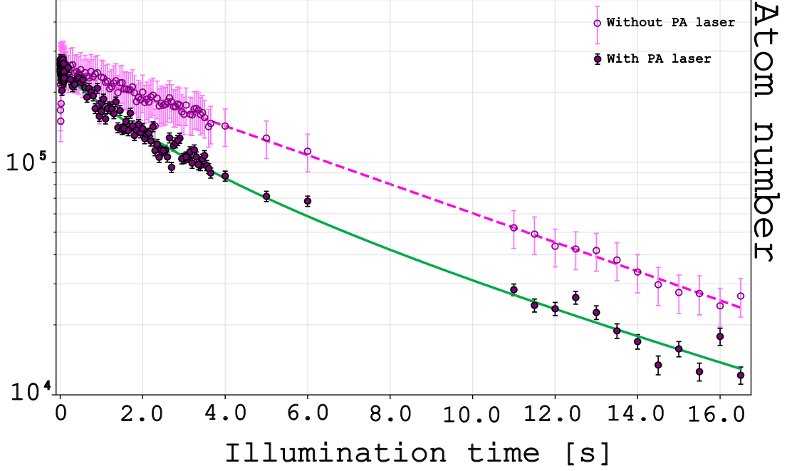
Figure 3.19: Evolution of the atom number (on a logarithmic scale) as a function of the illumination time, measured at a fixed laser detuning of f = -6 MHz from the atomic resonance (see Section 3.2.3.5). Filled circles represent the data in the presence of the photoassociation (PA) laser, adjusted with the fit function (Eq. 3.82) accounting for combined one- and two-body losses. Open circles display the reference measurement at the same frequency in the absence of the PA laser. The distinct decay behaviors observed between the two datasets highlight that relying solely on a single dN/dt decay measurement is insufficient to unambiguously characterize the loss mechanisms.
