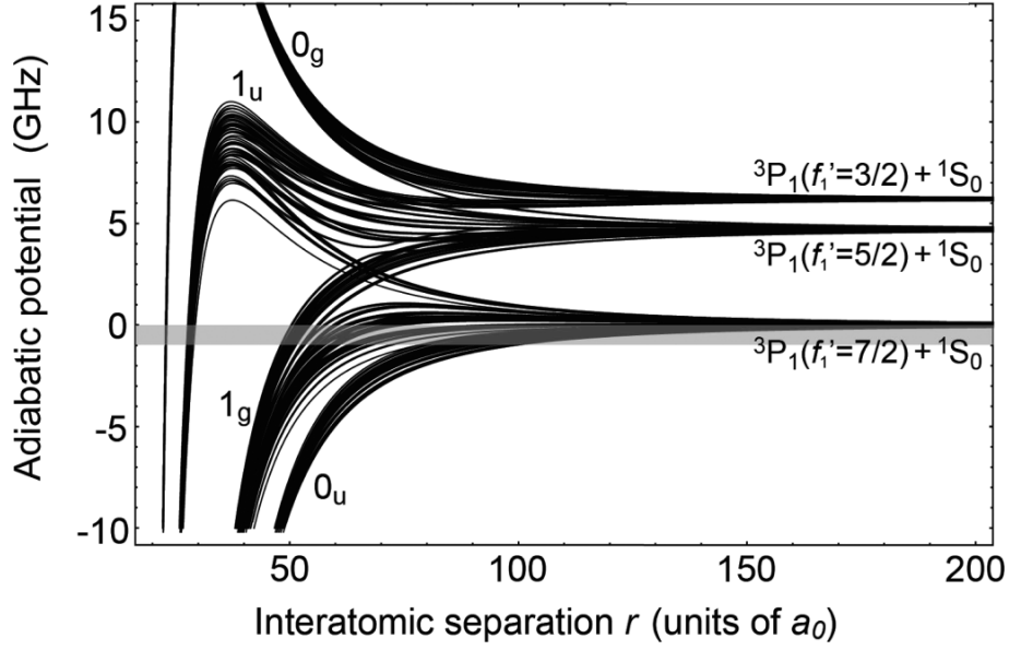
Figure 3.4: Density of molecular potentials for ^{173}\text{Yb} with three hyperfine states, giving rise to numerous triplets of quantum numbers ( T, F, R ). The spectral lines are identified as \Omega_{u/g} , where \Omega is the total orbital momentum projection of the molecule and u/g denotes the electronic parity (see Fig. ??).
