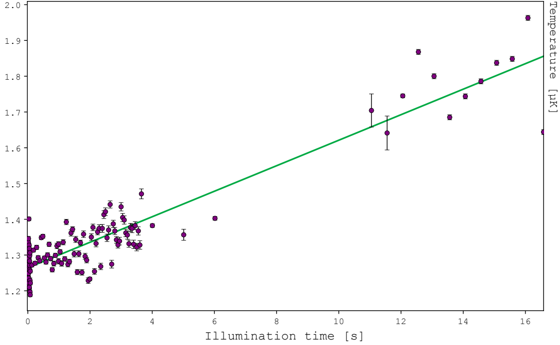
Figure 3.20: Temperature of the gas during the experiment described in Fig. 3.15, where the atom number decays with a two-body-loss-like behavior despite the signal being of atomic, not molecular, origin. The temperature increases linearly rather than following the saturating exponential expected for genuine photoassociative (two-body) loss, consistent with ordinary photon-scattering heating rather than molecule formation.
