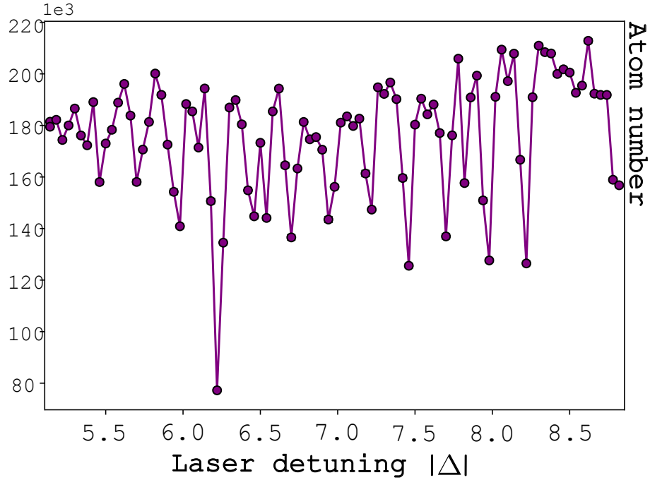
Figure 3.15: Atom number measurement on ^3P_1, F = 11/2 hyperfine excited state, measured in an SU(10) gas at \delta = +6 MHz from the atomic resonance. This heating-broadened pattern of single-atom lines is obtained by a sideband in the diode laser spectrum that is addressing the atomic resonance.
