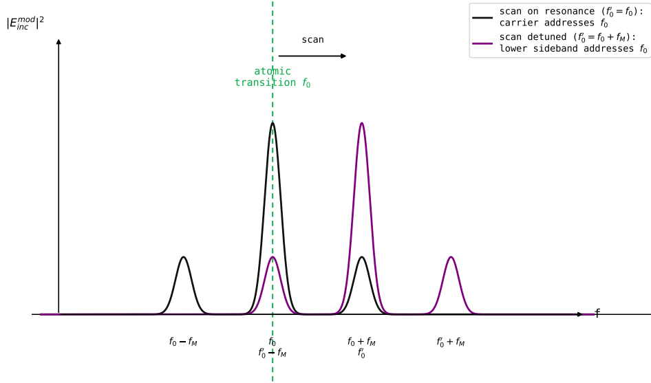
Figure 3.11: Scheme of the PDH sidebands addressing the atomic resonance, shown at two snapshots of the laser frequency scan. The atomic transition sits at the fixed frequency f_0 (green dashed line). In black: the carrier is scanned onto resonance ( f'_0 = f_0 ), producing the true photoassociation signal. In purple: the carrier is instead detuned to f'_0 = f_0 + f_M , so that it is itself off-resonance, but its lower sideband coincides with f_0 and drives a spurious ("ghost") loss resonance. As the scan sweeps f'_0 , this coincidence recurs whenever f'_0 = f_0 \pm f_M , producing satellite peaks such as the one reported in Fig. 3.12.
