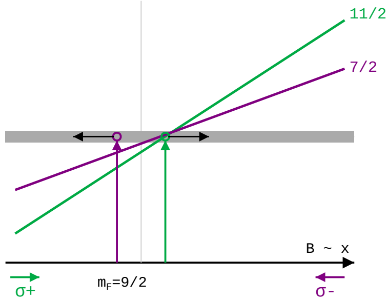
Figure 1.12: (Adapted from [30]) Illustration of the MOT effect on the m_F states of the hyperfine ^3P_1, F = 11/2 level. The position-dependent light shift brings the two counter-propagating beams into resonance with different m'_F sub-levels ( \sigma^+ with the closed transition to m'_F = 11/2 , \sigma^- with the open transition to m'_F = 7/2 ) at the same position, opening a leak out of the cycling transition.
