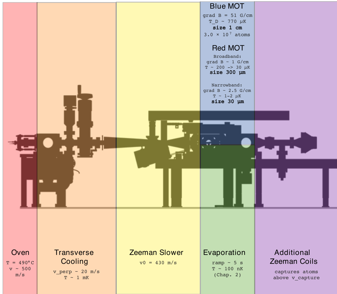
Figure 1.2: Extracted and modified from [22] Experimental full setup for the cooling and trapping of the atoms with figures on the velocity, temperature and typical magnetic gradient on each stage.
