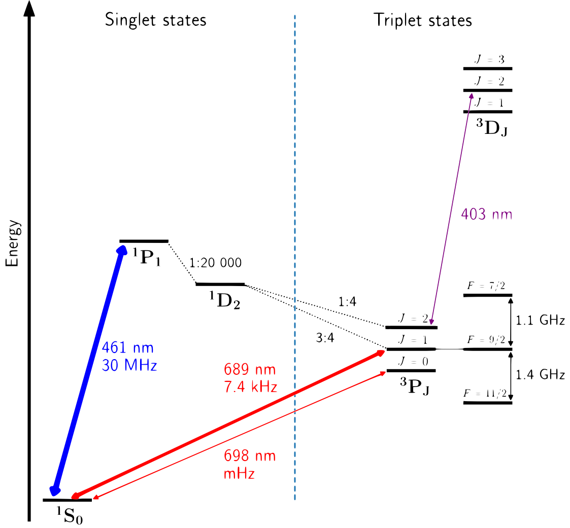
Figure 1.1: Extracted from [21] Energy spectrum of ^{87}\text{Sr} including fine and hyperfine interactions. In blue the 461 nm transition used for TC, Zeeman cooling, blue MOT stage and imaging. The purple arrow indicates the repump line at 403 nm from the metastable state ^3P_2 used for the atoms leaking from the intermediate ^1D_2 state. In red the transition to ^3P_1 at 689 nm used for all stages of the red MOT, optical pumping, spin manipulation, coherent manipulation (see Chap.2), photoassociation (see Chap.3, through the different hyperfine states F = 7/2, 9/2, 11/2 ). The 698 nm transition indicates the clock transition which we do not use in this experiment.
