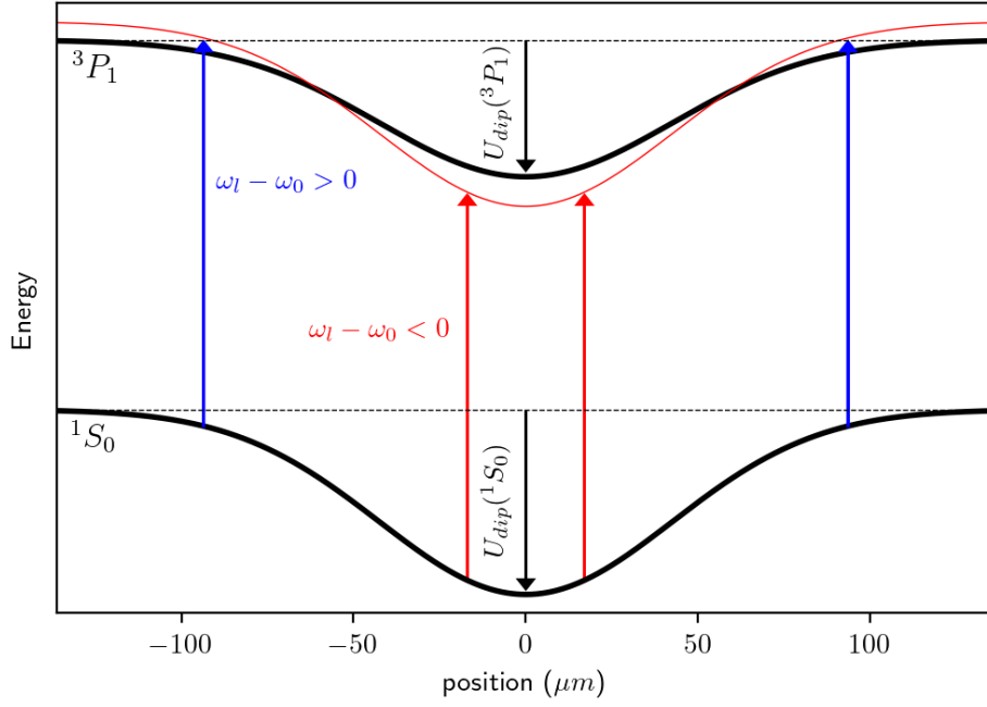
Figure 1.16: Simulation extracted from [21]. Principle of localized 689 nm MOT loading inside the crossed optical dipole trap due to the differential AC Stark shift between ^1S_0 and ^3P_1 .
