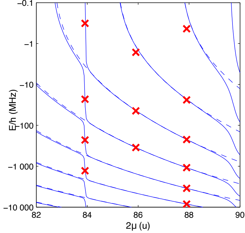
Figure 3.7: This graph - extracted from [11]- confronts the experimental internal states in red crosses to their theoretical predictions for different reduced mass of strontium isotopes. The theoretical model guarantees approximated scales for molecular lines of ^{87}\text{Sr} but not precisely because this model neglects the hyperfine interaction of the species.
