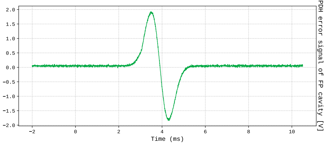
Figure 1.26: Pound-Drever-Hall (PDH) error signal obtained by scanning the cavity length across resonance, enabling the lock cavity for the filtering of MOGlabs laser.
