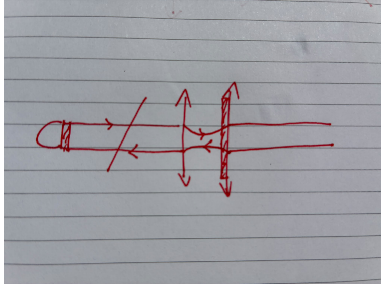
Figure 1.19: MOGlabs External Cavity Diode Laser (ECDL) architecture used for spin manipulation. A diode lasing at 689 nm is frequency settled by an interferential filter to then be collimated by a lens. The beam is focused in the middle of this lens and a second one where the beam is reflected: this system is selecting more precisely the frequency of the laser as a cateye.
