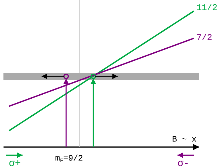
Figure 1.12: Counterpropagating lasers in resonance with lightshifted m_f states of ^3P_1, F = 11/2 hyperfine state.
