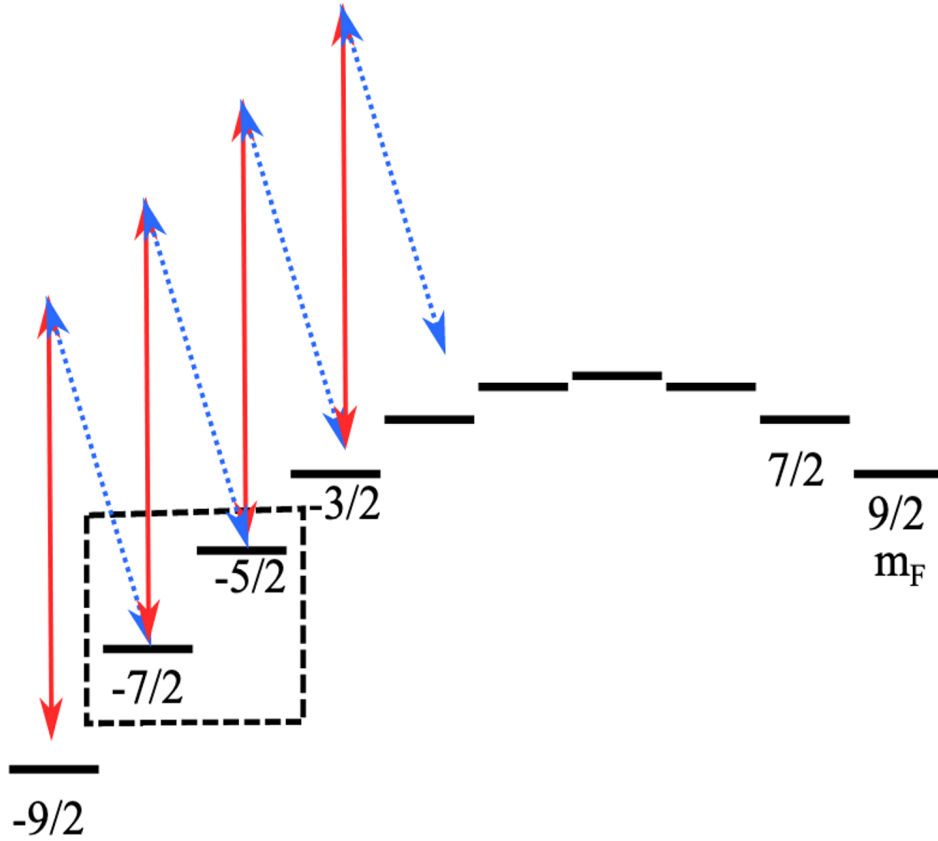
Figure 1.20: Spin manipulation scheme of [4]. The isolation of spin states is allowed by the tensorial shift of the ground states that makes neighbours m_F states isolated from the other resonances.
