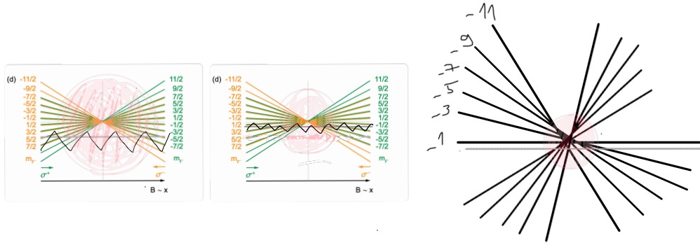
Figure 1.14: Sequential stages of the 689 nm red MOT. From left to right : swap cooling, broadband capture and single-frequency cooling (adapted from [? ]). The size of the cloud is decreasing with the cooling since the atoms are kicked in the opposite direction of the resonant laser of right polarization.
