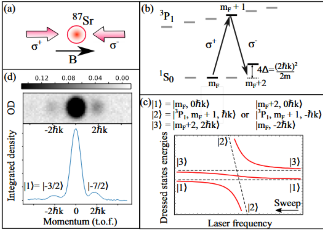
Figure 1.29: Principle of spin-selective detection via coherent momentum transfer. (a) Counter-propagating beam geometry of the lasers used for the TLS and two-photon Raman scheme. (b) Energy levels scheme of the Raman process, with recoil energy shifting the m_F + 2 level. (c) Avoided crossing due to the coupling of the states, necessitating adiabatic transfer. (d) Resulting TOF absorption image showing spatially separated spin components and the corresponding momentum distribution.
