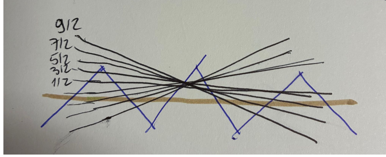
Figure 1.13: Illustration of the melange concept added to the red MOT cooling to capture extreme spin states components inaccessible from the counterpropagating lasers of the red MOT.
