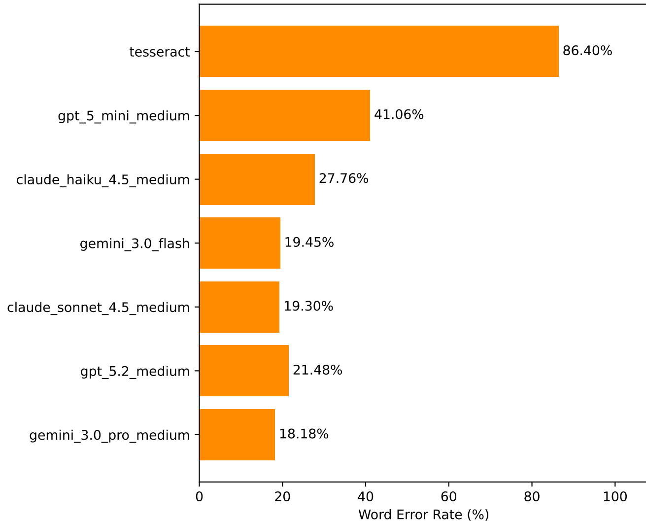
WER by Model (Lower is Better)
