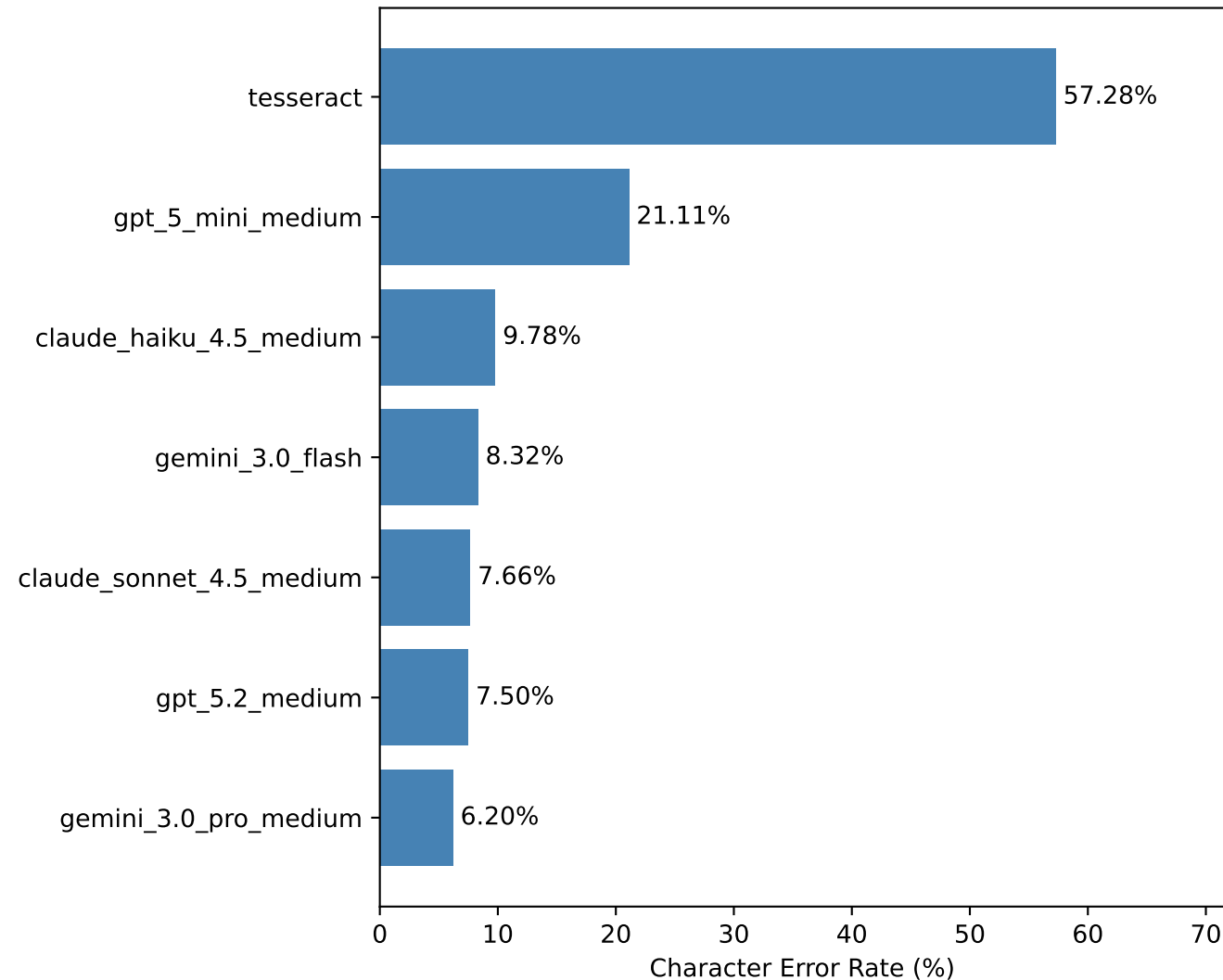
CER by Model (Lower is Better)
