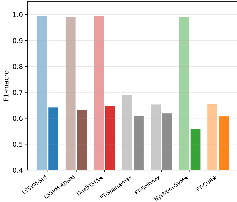
Dataset: TWS
