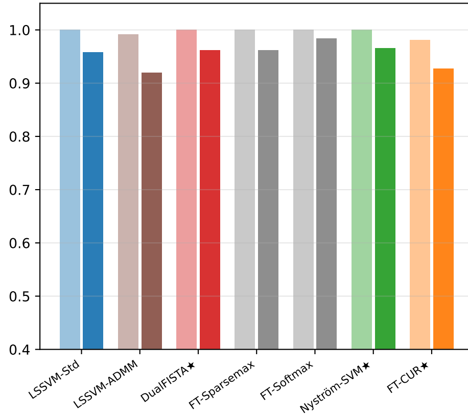
Dataset: TWM
