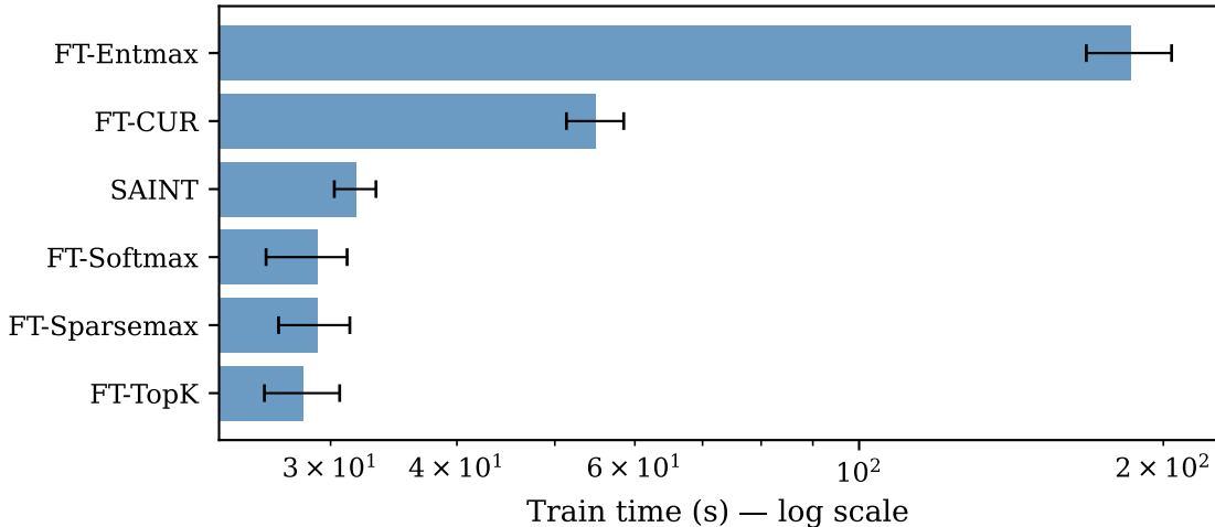
Median training time per model (IQR bars)
