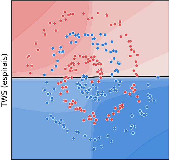
FT-Softmax (inter-atributos)
