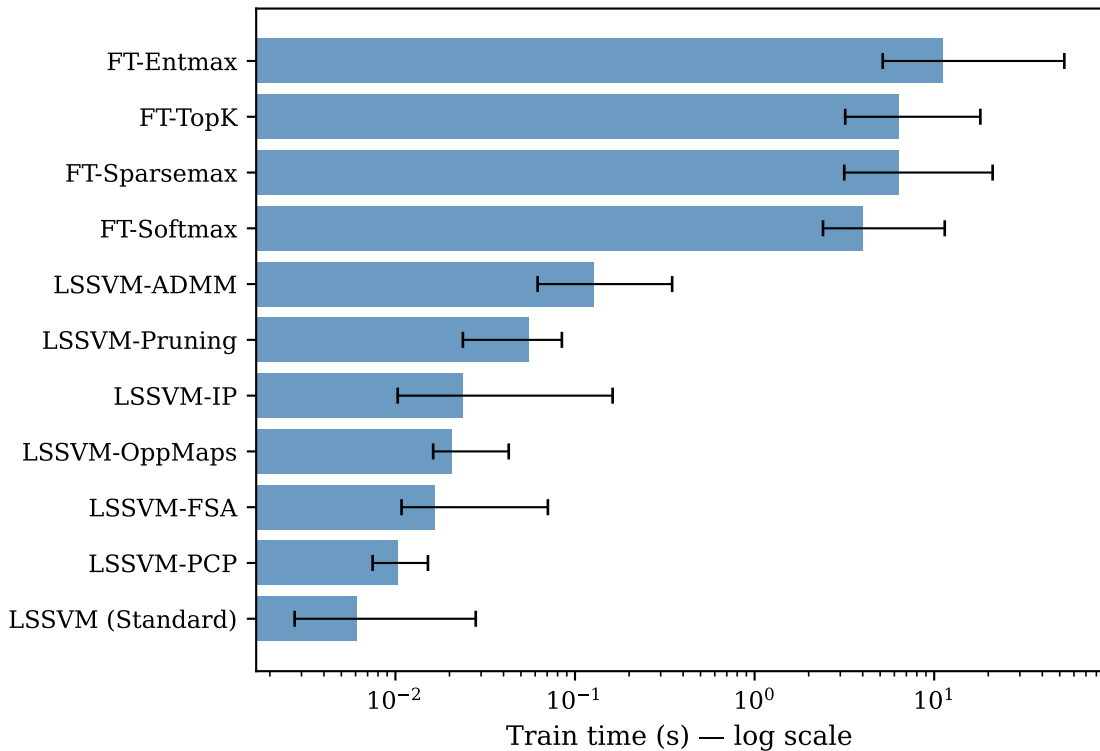
Median training time per model (IQR bars)
