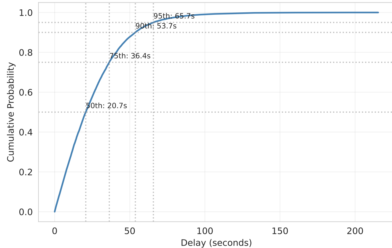
Cumulative Distribution Function (CDF) of Delays
