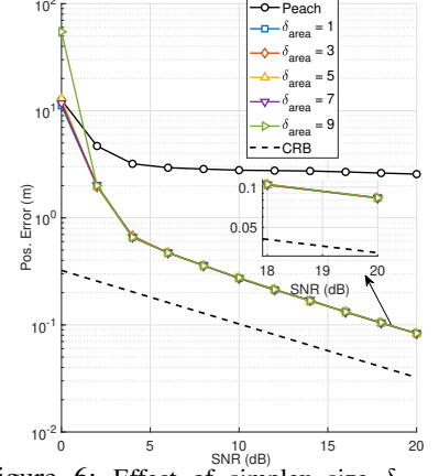
Figure 6: Effect of simplex size \delta_{\text{area}} on PEACH-NM performance.
