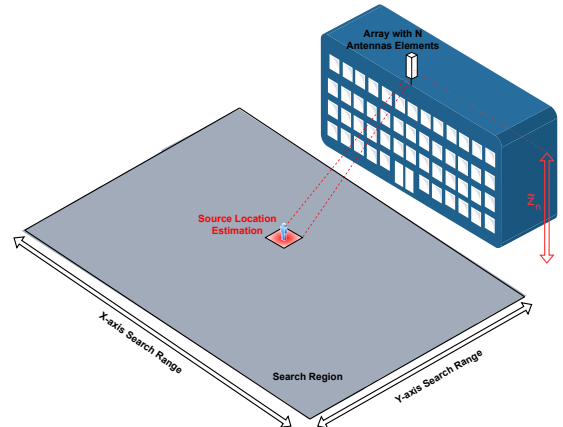
Figure 1: Representation of the elevated antenna array with the user located on the ground-level xy -plane.
