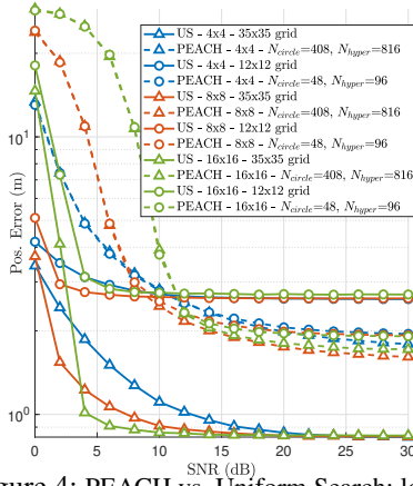
Figure 4: PEACH vs. Uniform Search: localization error under different array sizes and complexities.
