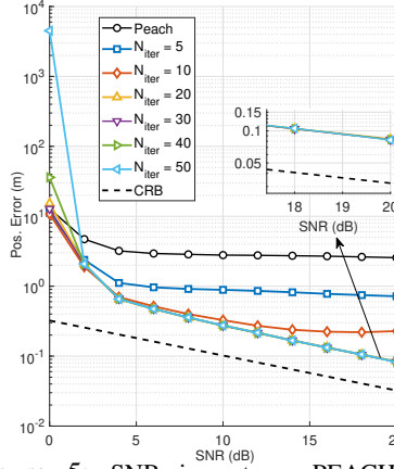
Figure 5: SNR impact on PEACH and PEACH-NM accuracy: CRB as baseline.
