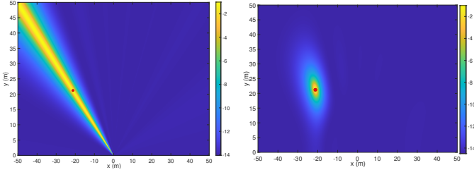
(a) Antennas at user height ( \tilde{z}_n = 0 ) (b) Antennas elevated ( \tilde{z}_n = 20 m)
