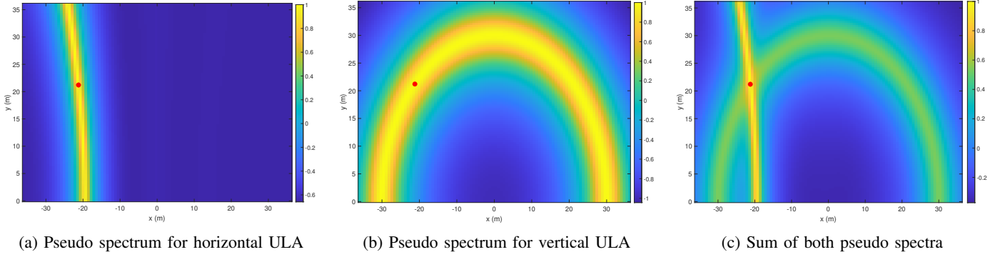
Figure 3: MUSIC pseudo spectra for a single user at 30 m in the xy-plane using an 8 \times 8 URA at 15 GHz (SNR = 15 dB, elevation \tilde{z}_n = 50 m): (a) Horizontal ULA ( 1 \times 8 ), (b) Vertical ULA ( 8 \times 1 ), and (c) Sum of pseudo spectra.
