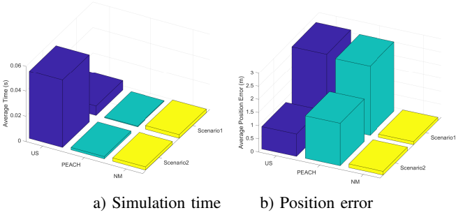
Figure 7: Simulation time and Localization error for Uniform Search and PEACH-based estimators
