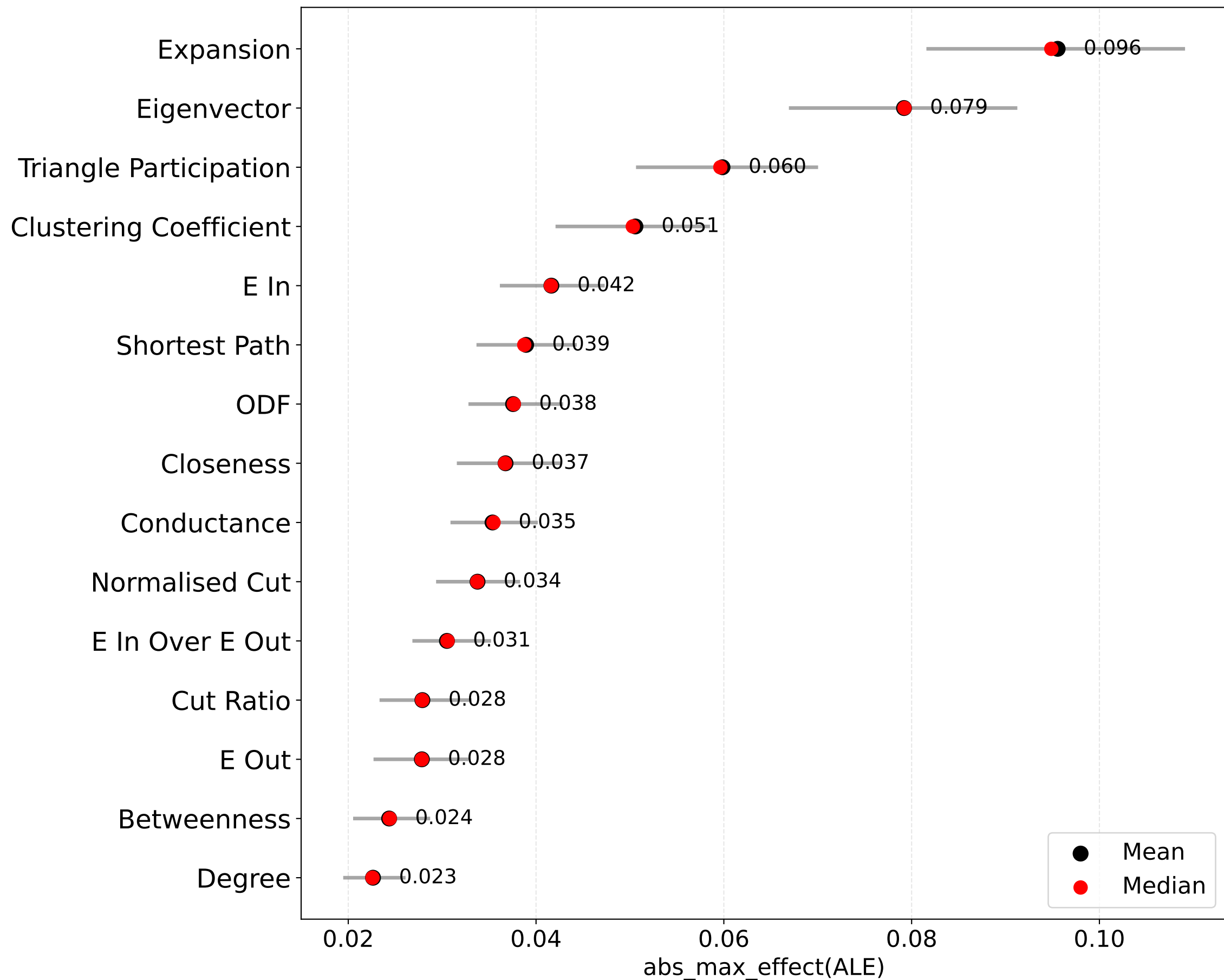
Louvain, \mu = 3
