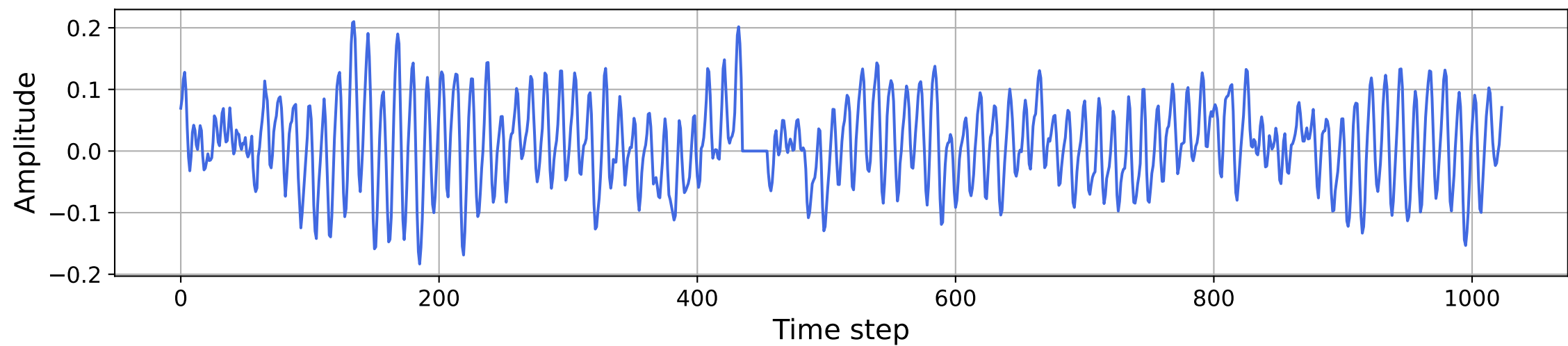
Class 1
