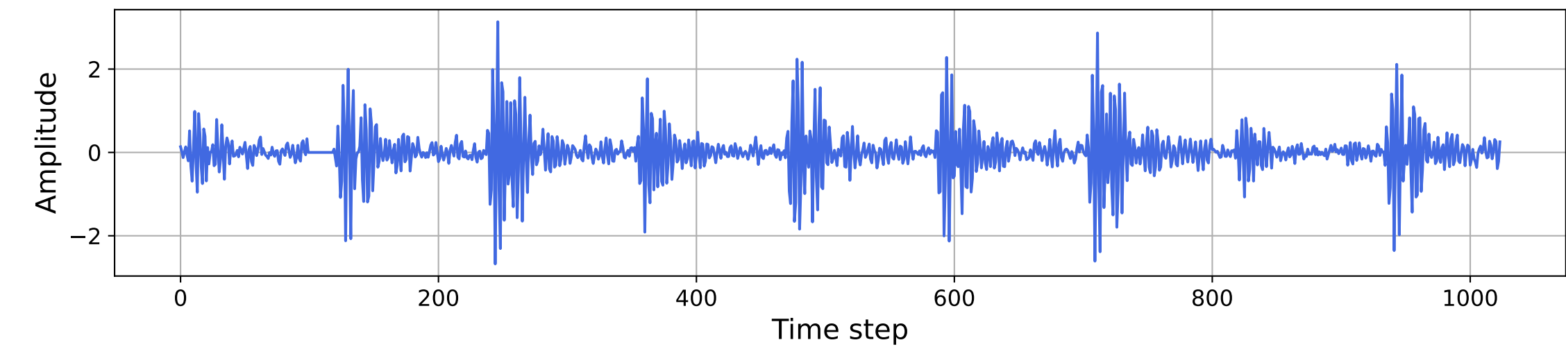
Class 3
