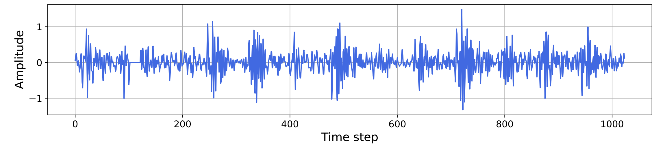
Class 2
