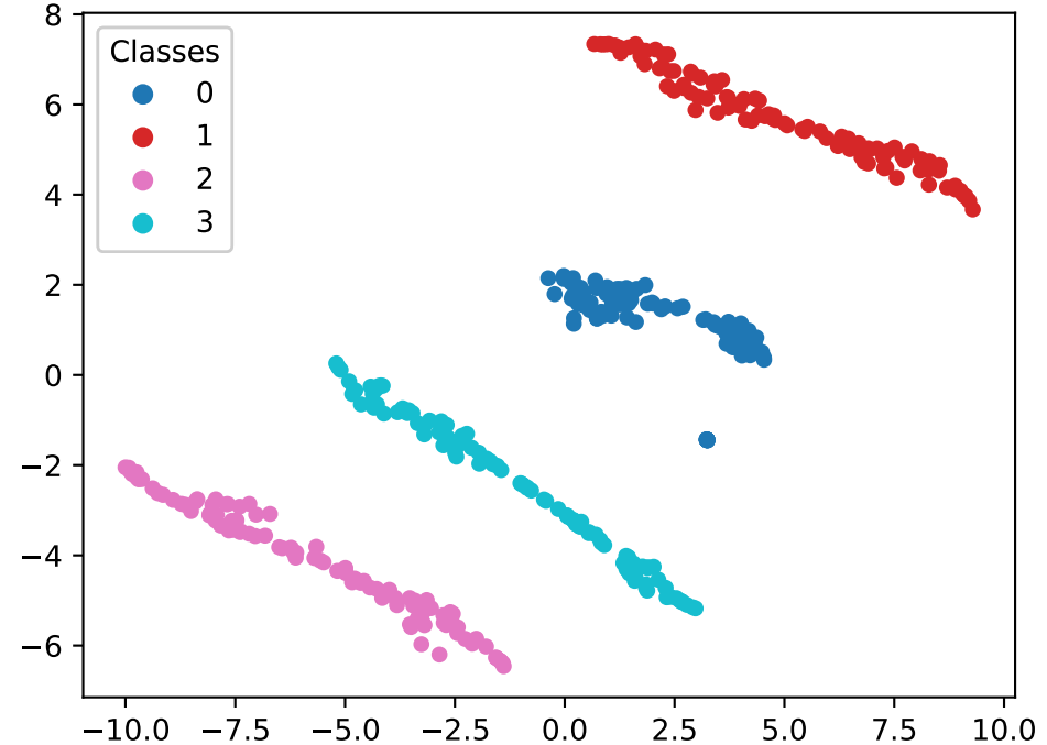
Dim 2 vs 3
