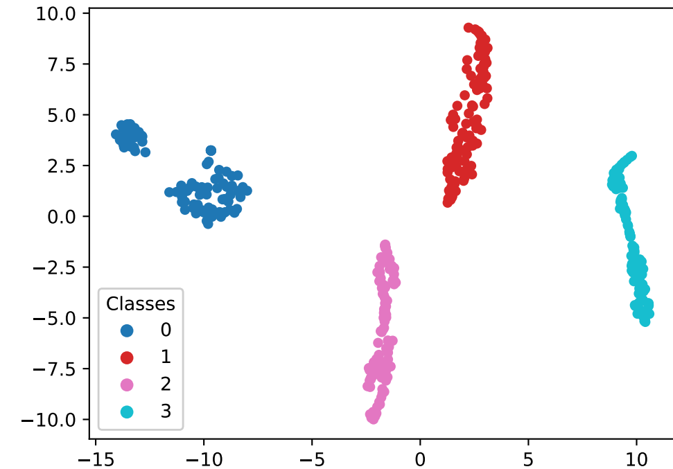
Dim 1 vs 2
