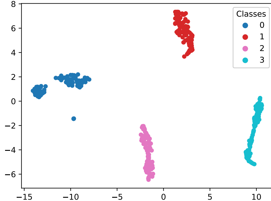
Dim 1 vs 3
