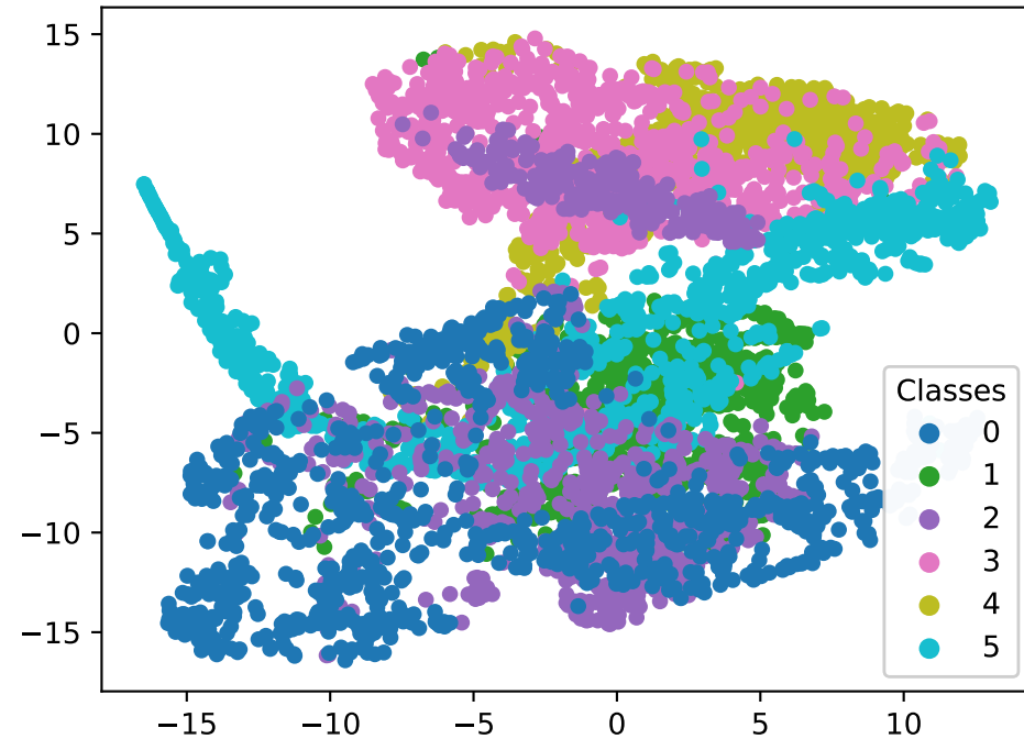
Dim 2 vs 3
