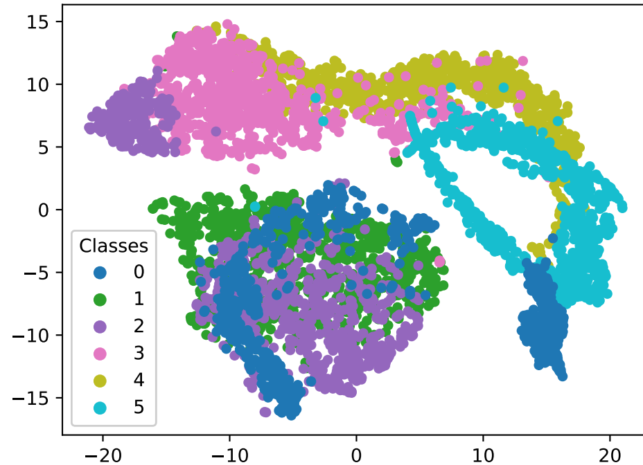
Dim 1 vs 3
