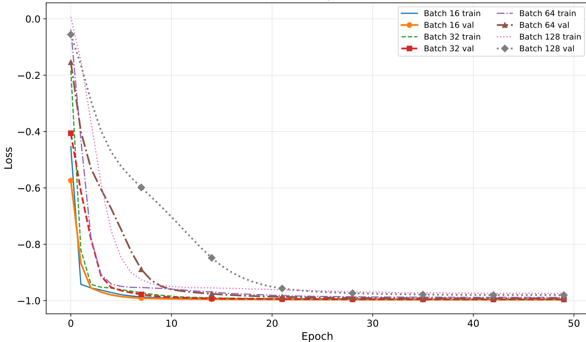
Train vs validation loss by batch size (means)
