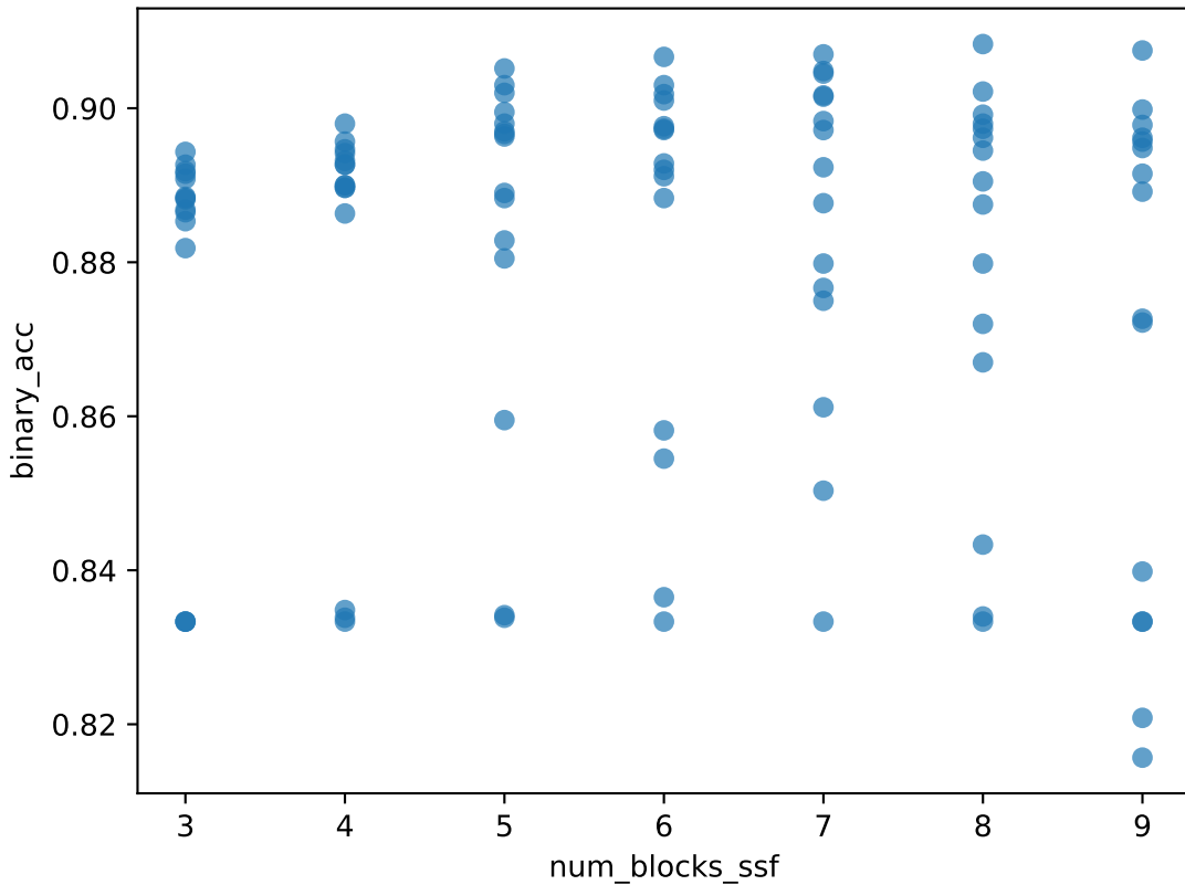
num_blocks_ssf vs Best Binary Accuracy
