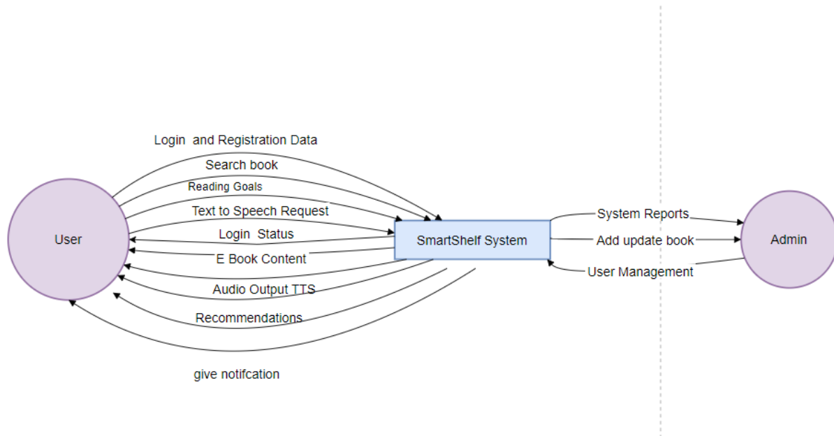
Figure 39 DFD 0
