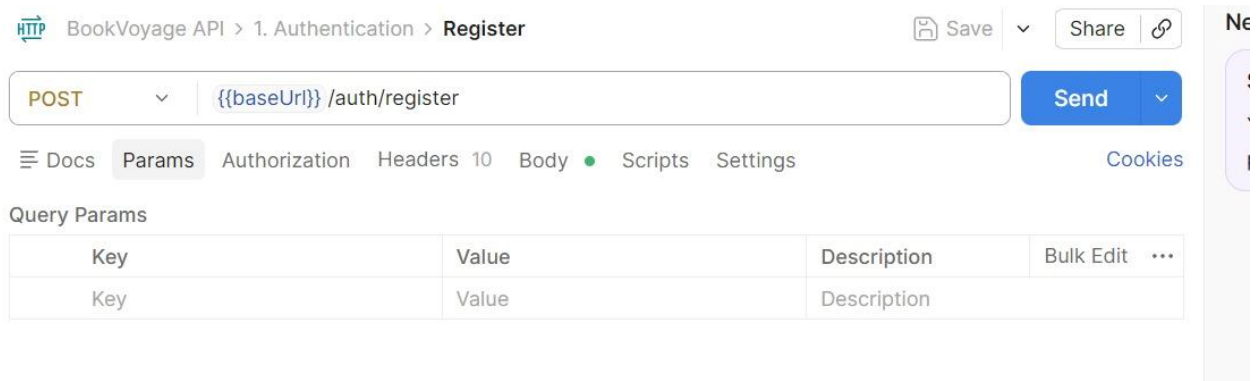
Figure 272 API Test 1
