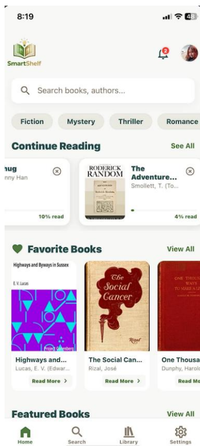
Figure 256 Reading Process
