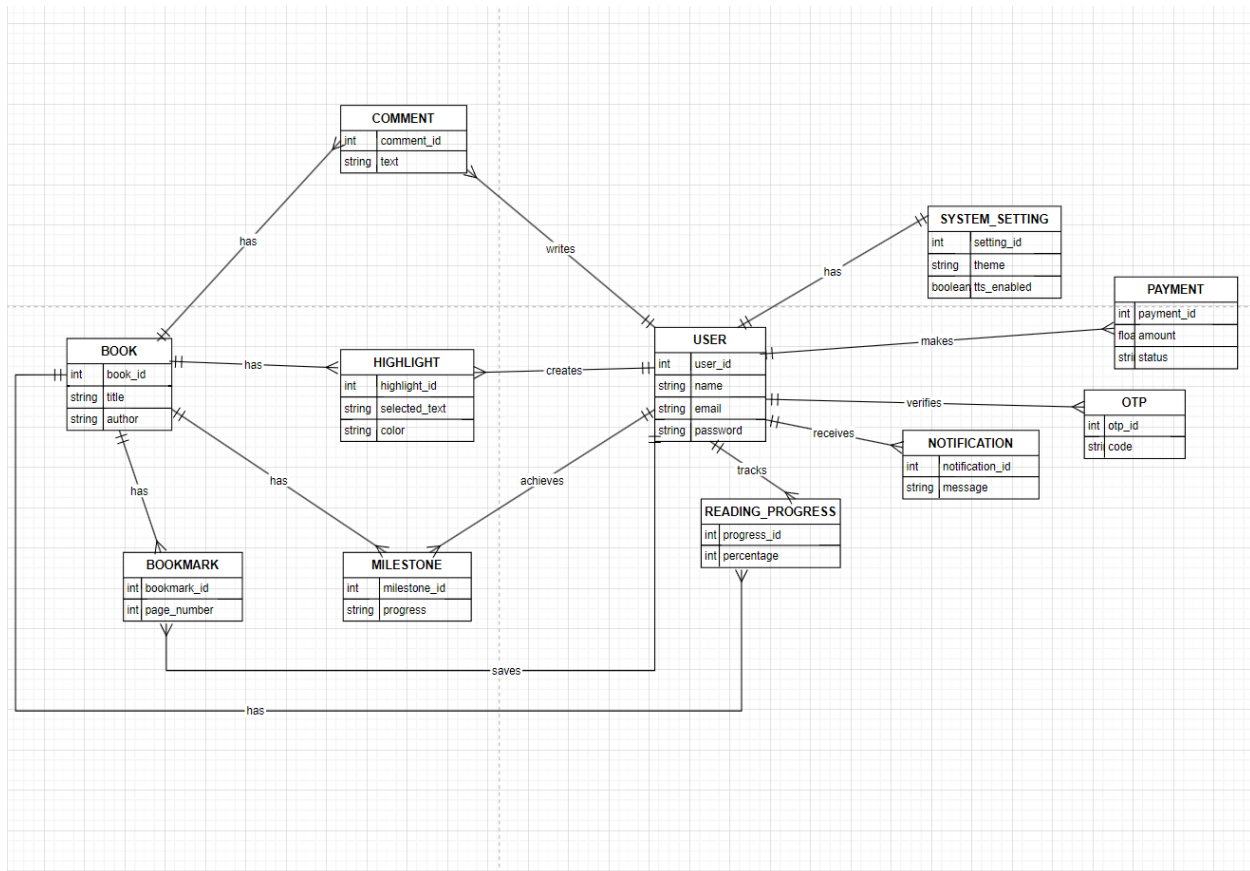
Figure 32 Final ERD
