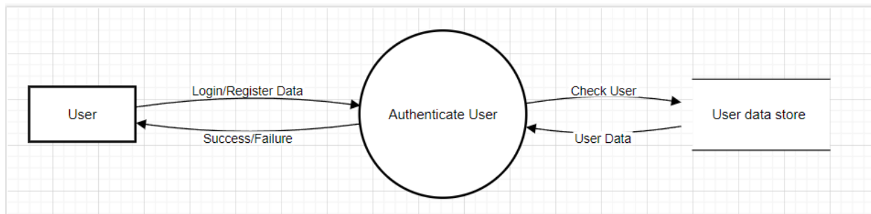
Figure 40 User Auth
