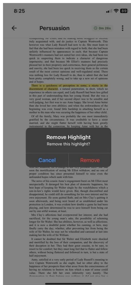
Figure 157 Remove Highlight
