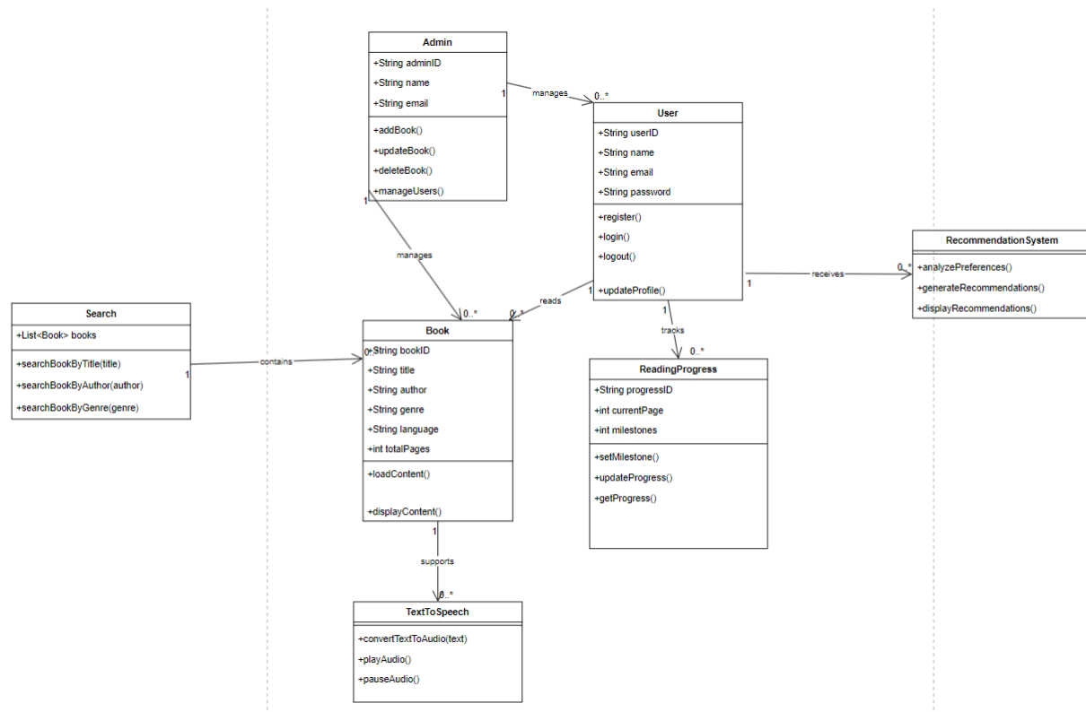
Figure 91 Class Diagram
