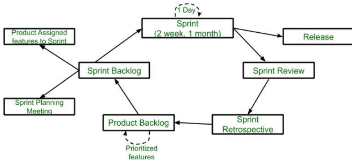
Figure 293 Scrum (GeeksforGeeks, 2025)
