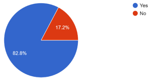
Figure 289 Question 5 Response
