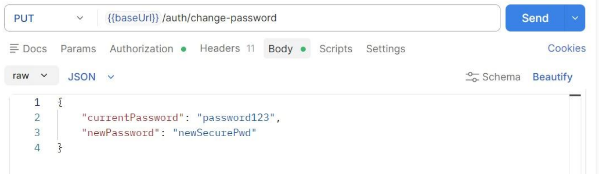
Figure 278 API Test 7
