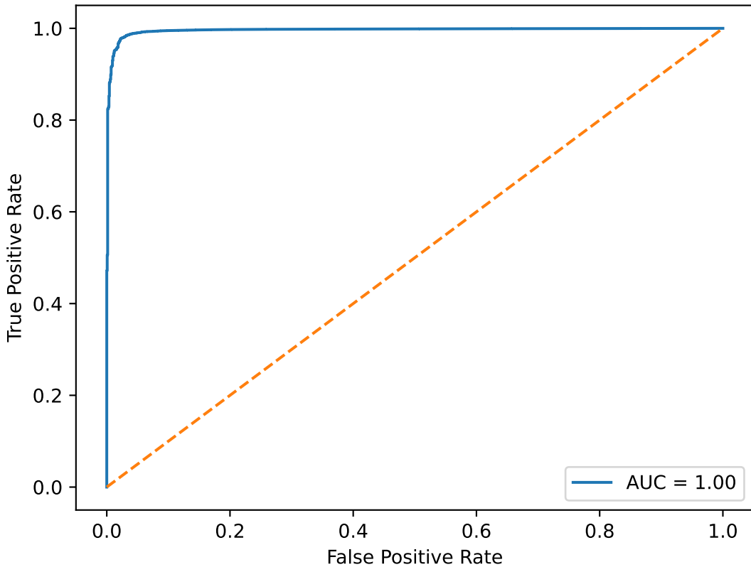
ROC Curve (Default vs Non-default)
