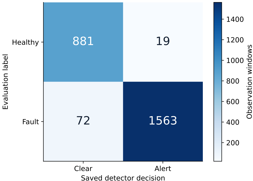
GRU: RCAEval window decisions
