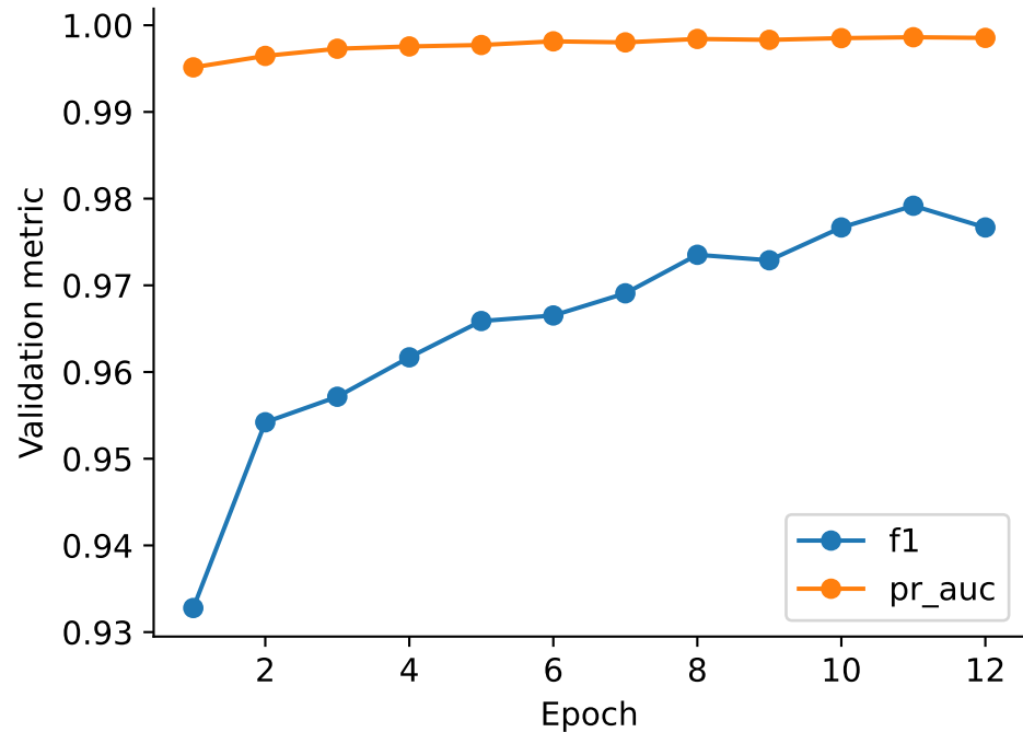
Recorded validation history
