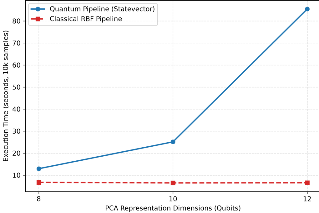
Figure 5: Measured Pipeline Execution Time Across Representation Dimensions
