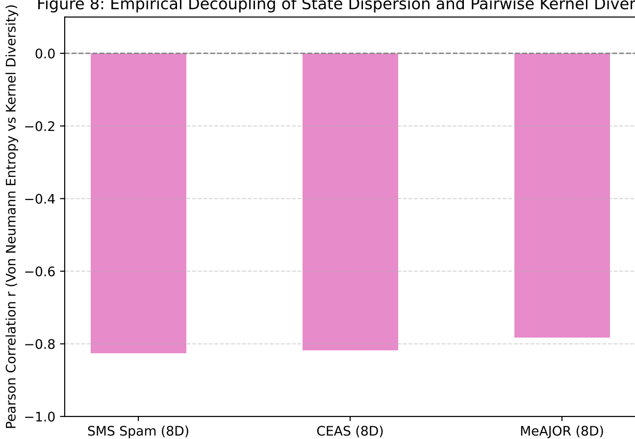
Figure 8: Empirical Decoupling of State Dispersion and Pairwise Kernel Diversity
