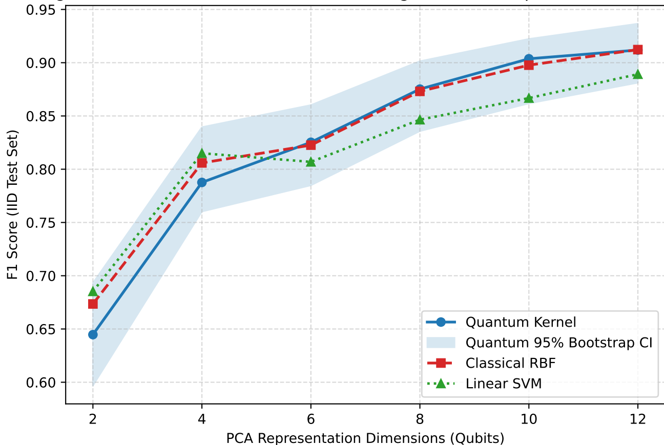
Figure 2: In-Distribution Performance Scaling with Bootstrap Confidence Band
