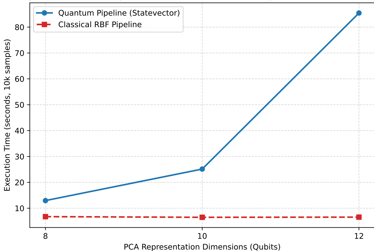
Figure 5: Measured Pipeline Execution Time Across Representation Dimensions
