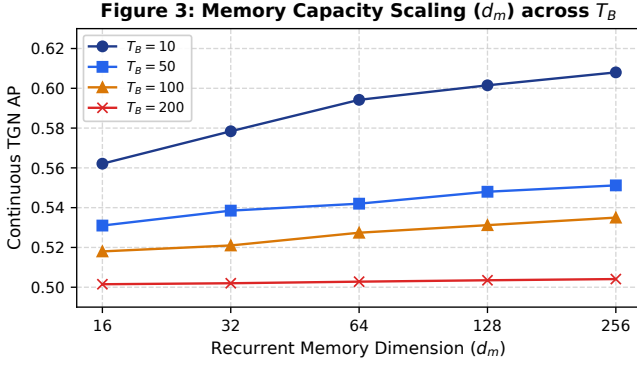
Figure 3: Recurrent Memory Capacity Scaling ( d_m ) across Distractor Durations T_B . Expanding continuous node memory dimension from d_m = 16 to d_m = 256 yields marginal gains without overcoming the unfeatured representation floor.
