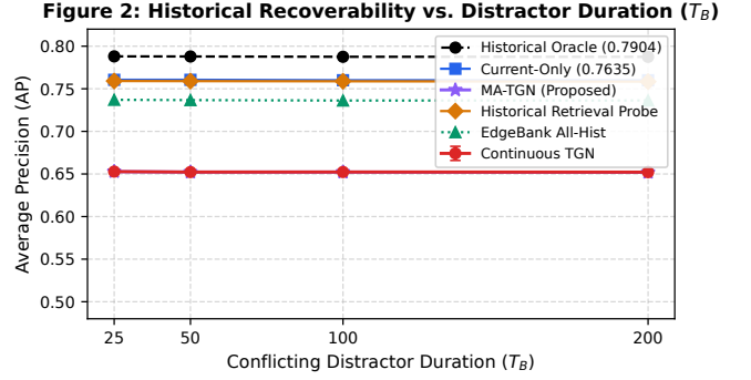
Figure 2: Historical Recoverability vs. Distractor Duration ( T_B ). Dynamic link prediction AP across T_B \in \{25, 50, 100, 200\} (10 random seeds). Statistical probes and deterministic baselines are compared against continuous neural models.
