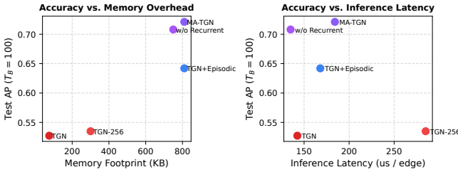
Figure 10: Accuracy vs. Memory and Latency Tradeoff ( T_B = 100 ).
