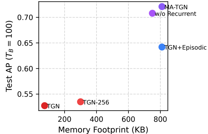
Accuracy vs. Memory Overhead
