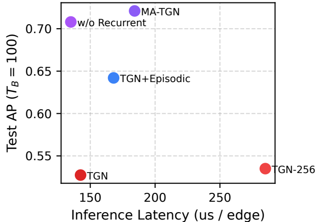
Accuracy vs. Inference Latency
