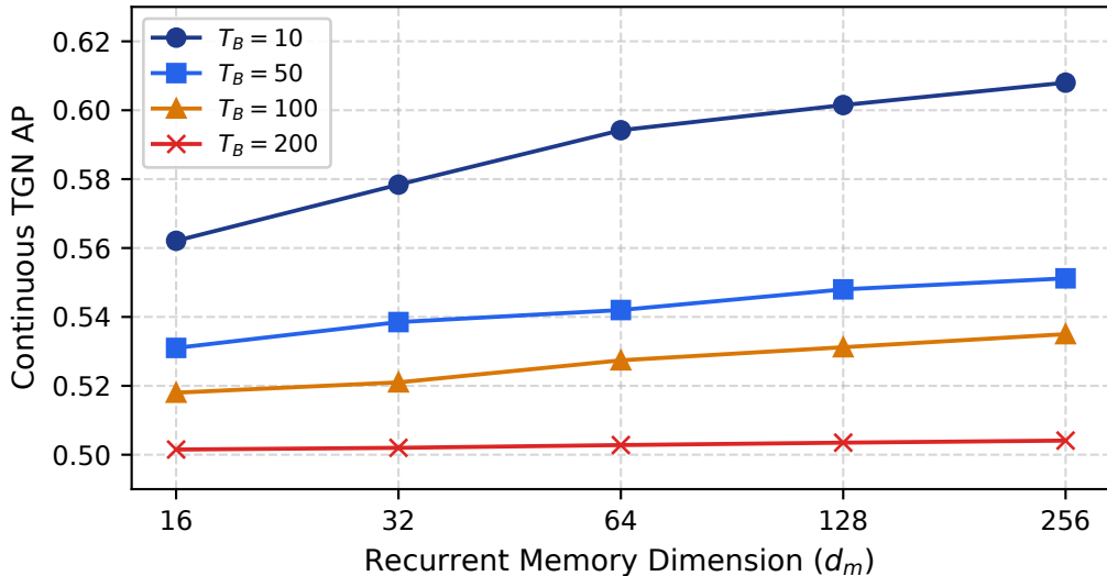
Figure 3: Memory Capacity Scaling ( d_m ) across T_B
