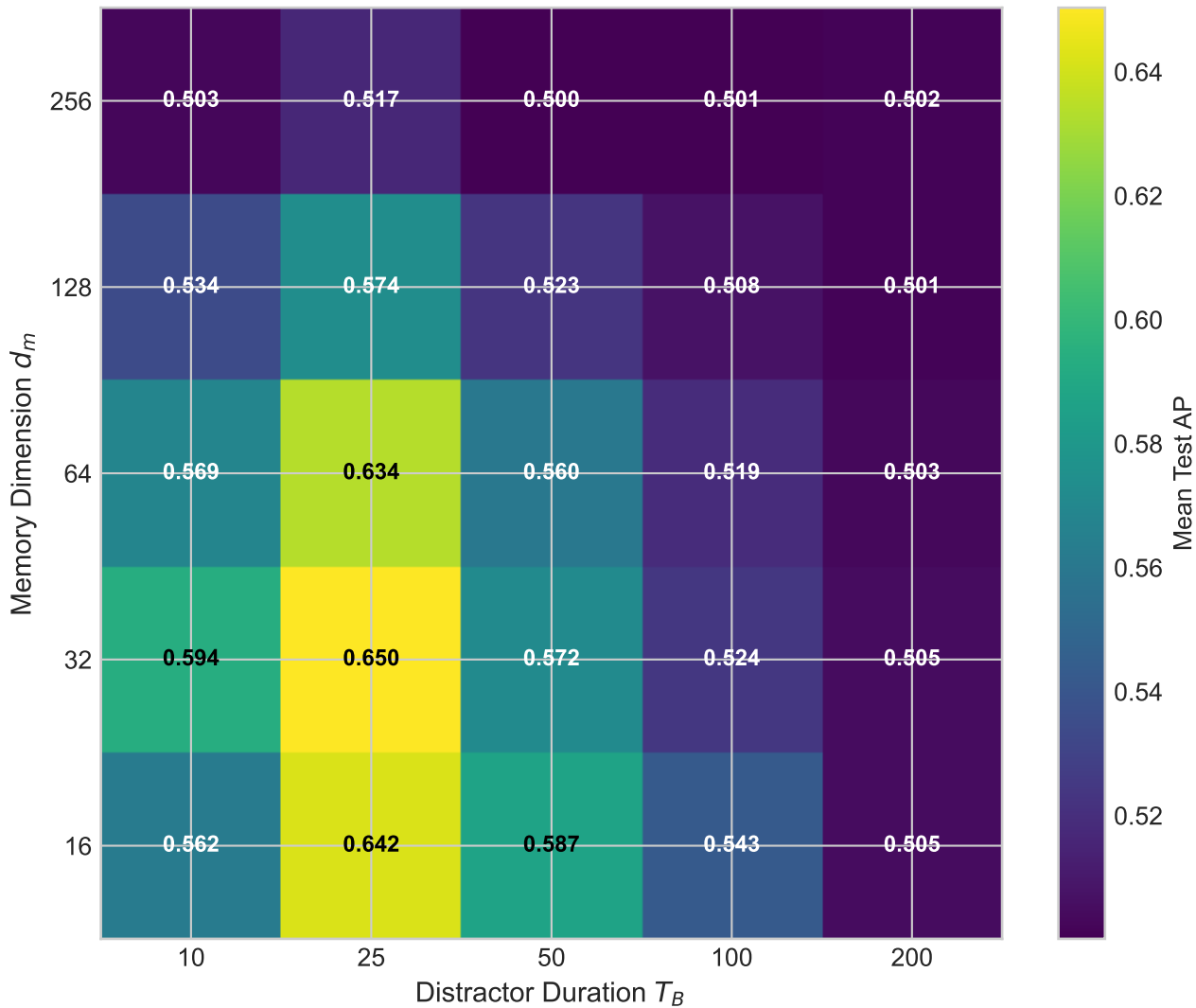
Figure 1: Recurrence AP across Memory Dimension and Distractor Duration
