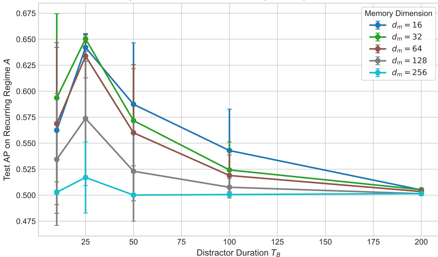
Figure 3: Recurrence AP vs T_B by Memory Dimension
