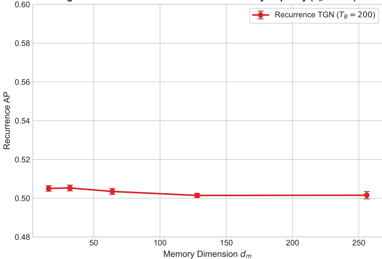
Figure 6: Recurrence Performance vs Memory Capacity ( T_B = 200 )
