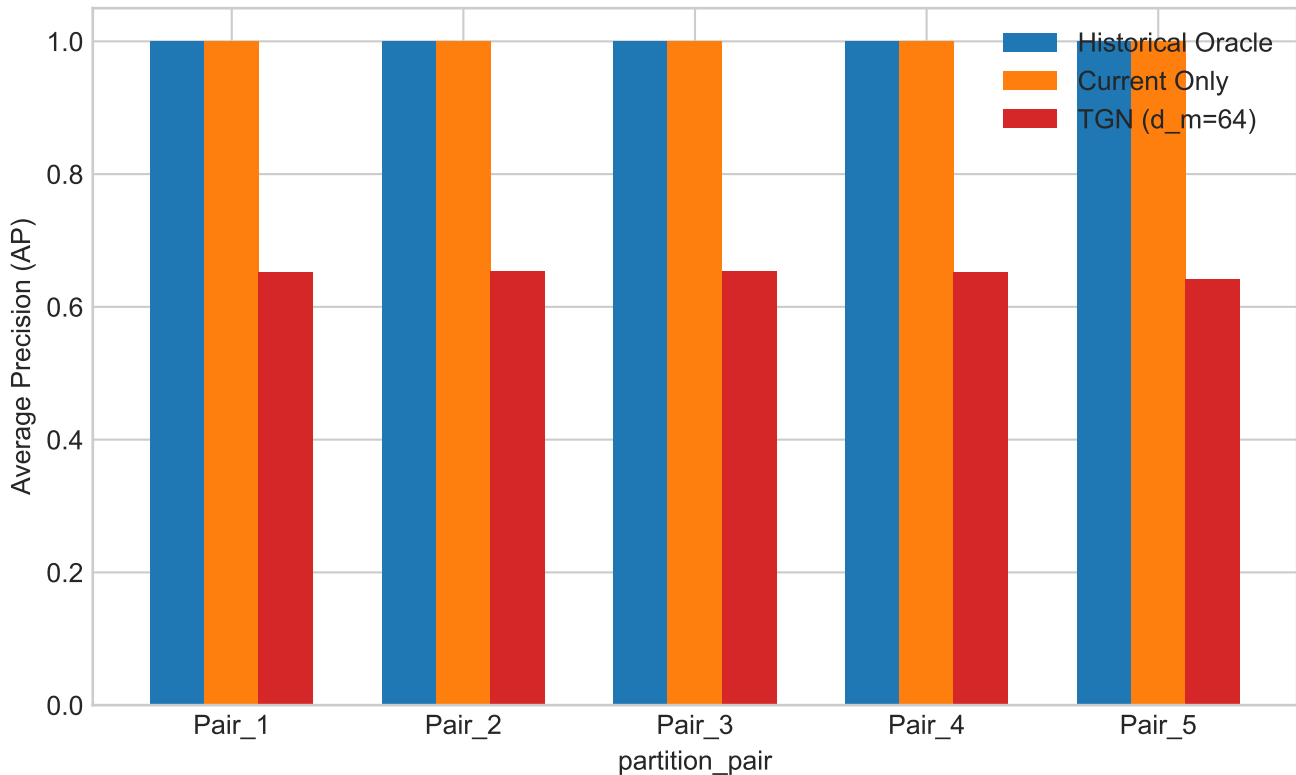
Figure 2: Invariance Across Orthogonal Partition Pairs
