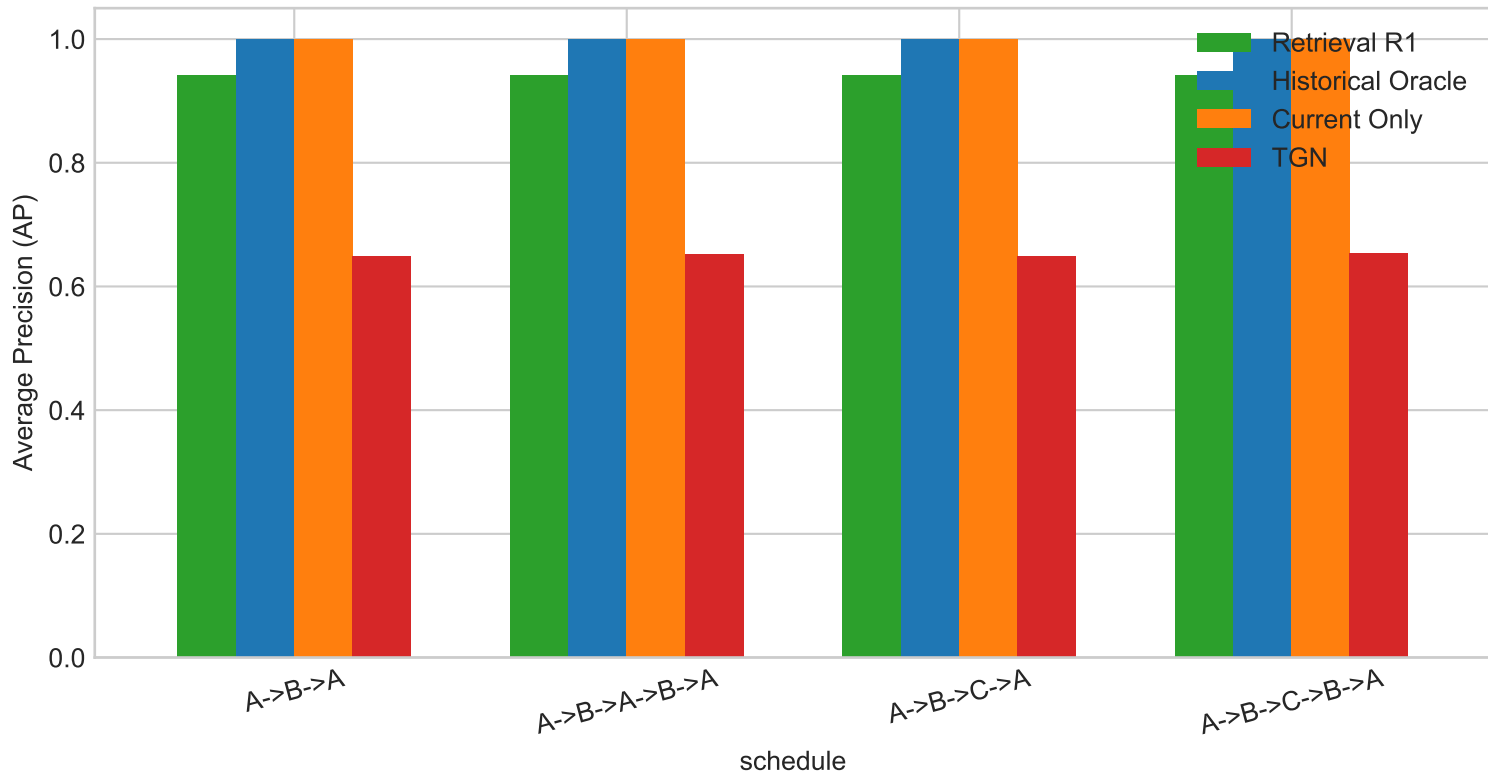
Figure 5: Generalization Across Multi-Cycle Recurrence Sequences
