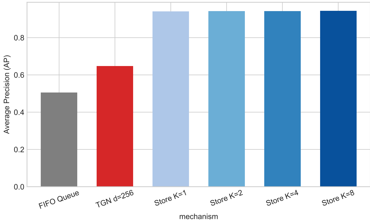
Figure 6: Memory Addressability vs Architecture Budget
