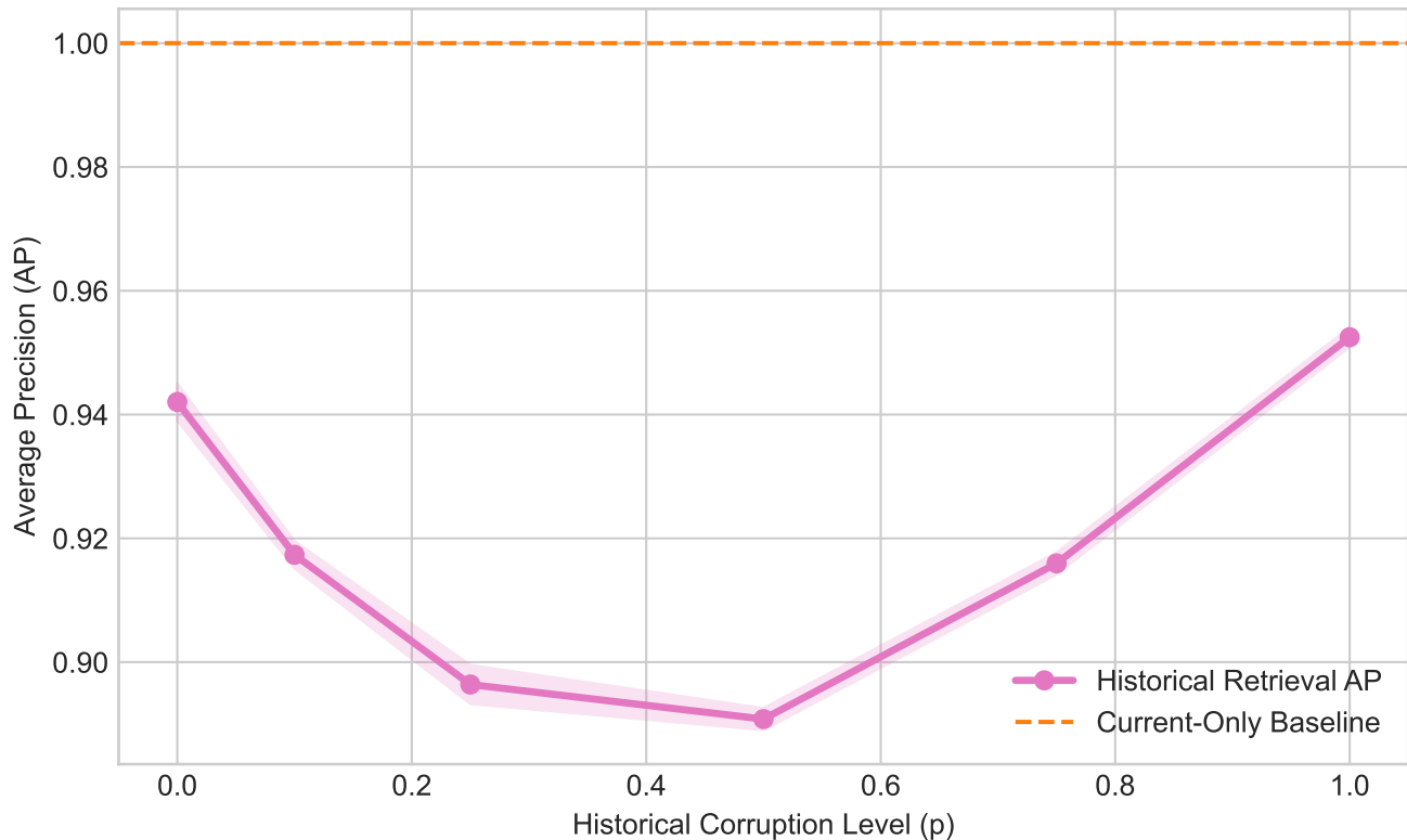
Figure 8: Retrieval Graceful Degradation under Historical Corruption
