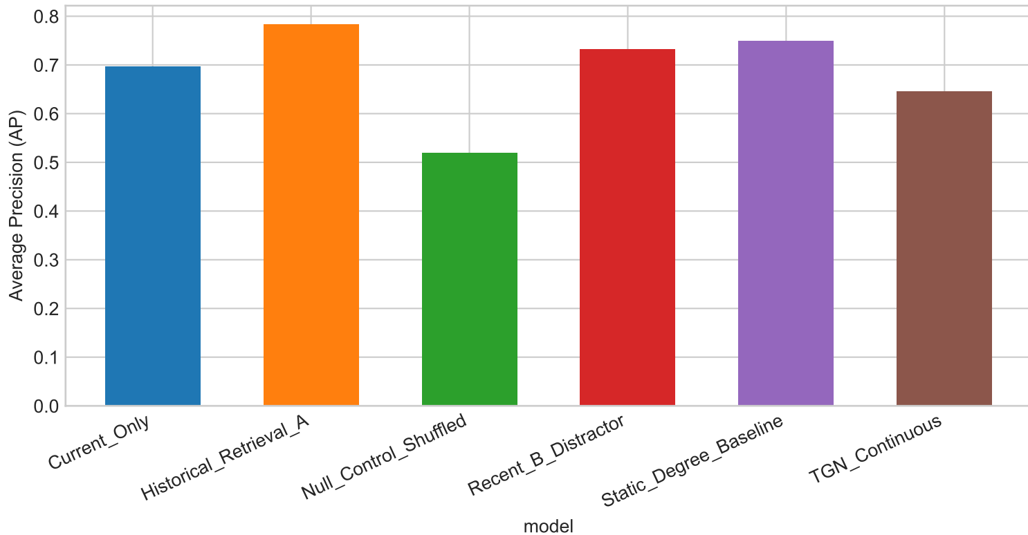
Figure 10: Model Comparison on Recurring SNAP CollegeMsg Episodes
