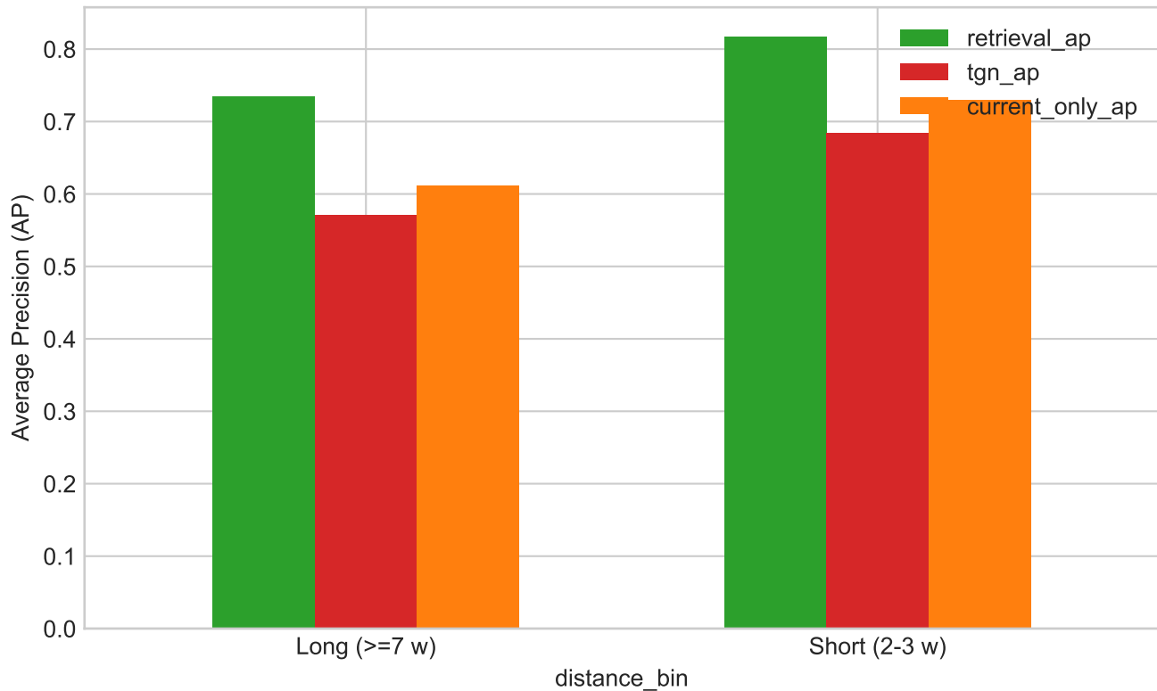
Figure 3: Performance vs Real Historical Distance Bins
