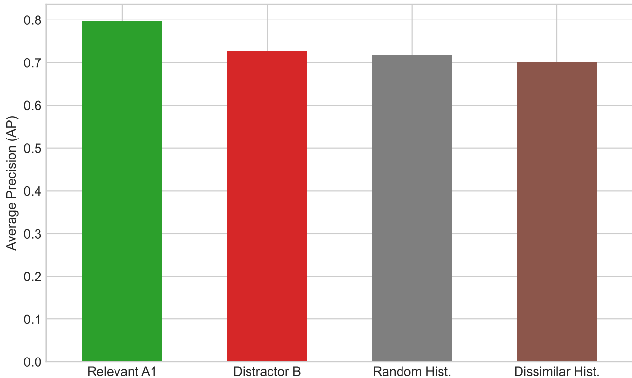
Figure 4: Real-Data Negative Controls vs Relevant Retrieval
