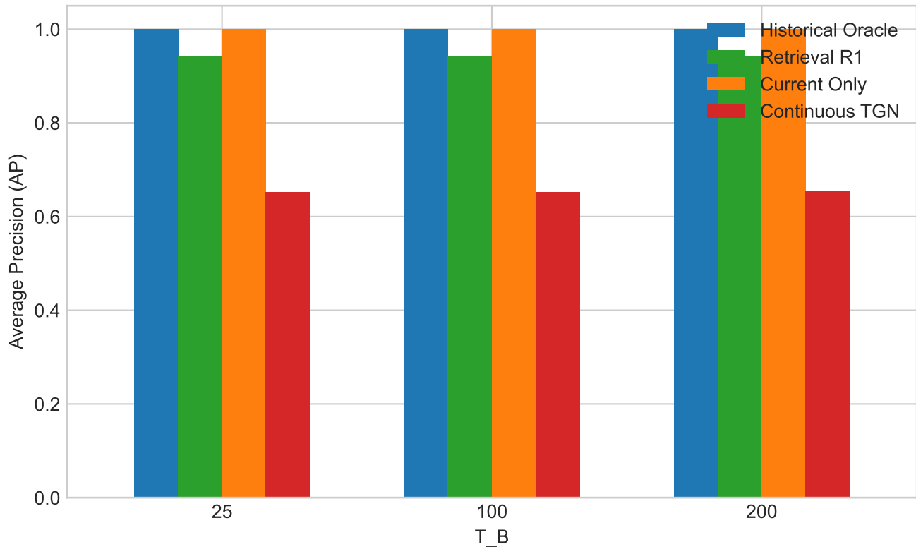
Figure 7: Final 10-Seed Synthetic Confirmation ( T\_B in \{25, 100, 200\} )
