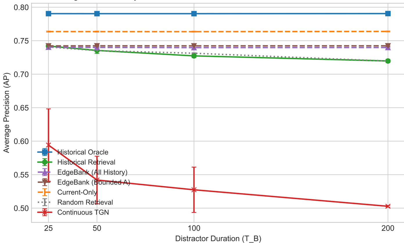
Figure 1: Hard Synthetic Benchmark Link Prediction vs Distractor Duration
