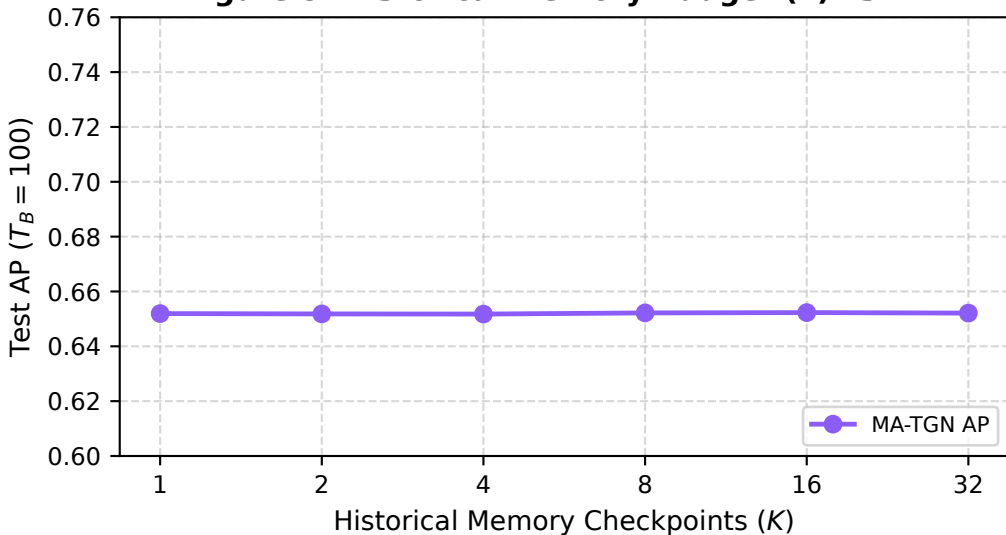
Figure 5: Historical Memory Budget ( K ) vs. AP
