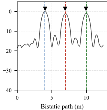
(c) Chirp-sequence FMCW, 2-D FFT
