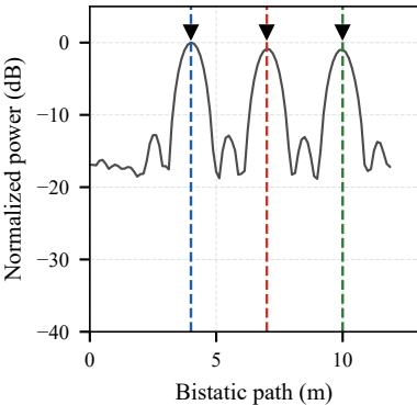
(a) M-FSK, 2-D processing
