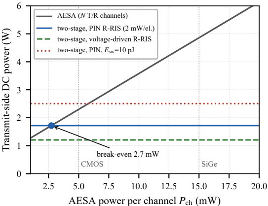
(a) N=256 ; common bistatic receiver excluded
