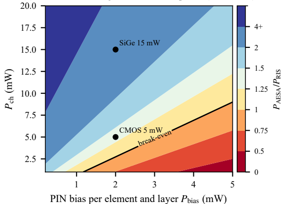
(b) Where the two-stage RIS draws less power (PIN R-RIS)
