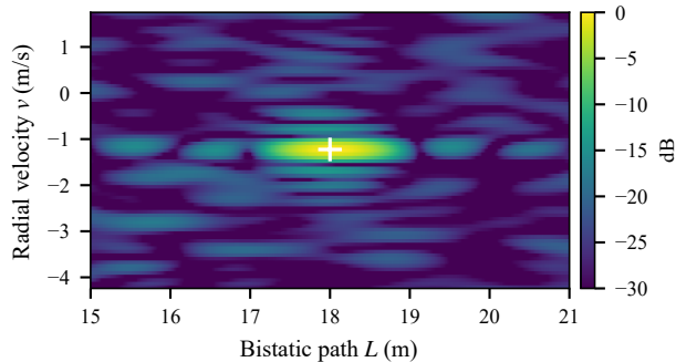
(b) Range-Doppler map (+: truth)
