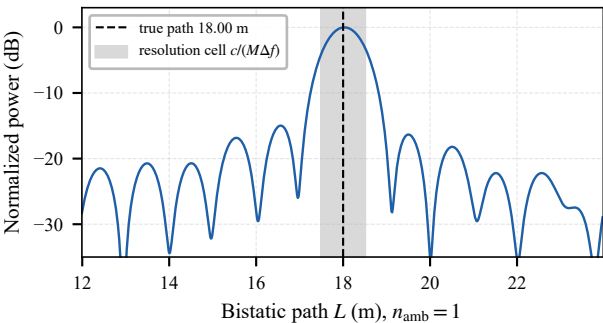
(a) IFFT path profile at the target Doppler
