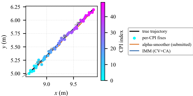
(a) Straight line, 2 m/s at 45^\circ (grey arrows: R-RIS beam)
