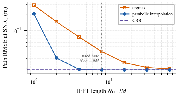
(b) Zero-padding versus interpolation (coherent processing)
