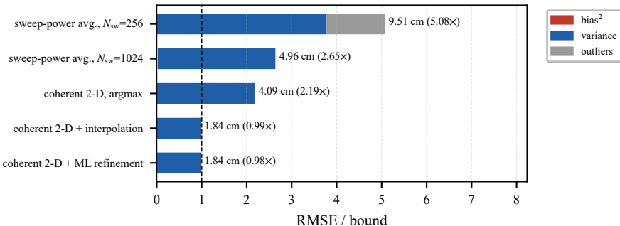
(a) Path RMSE / CRB at \text{SNR}_1 (bar split by MSE share)
